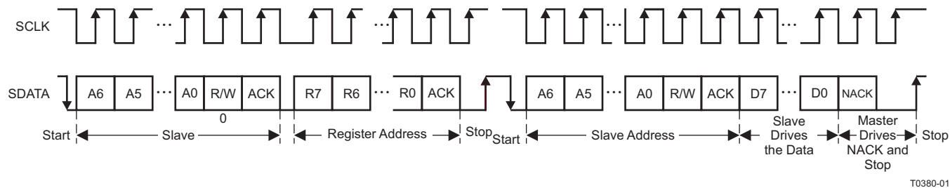
Figure 26. I²C-Bus Read From bq77PL900: Protocol B
