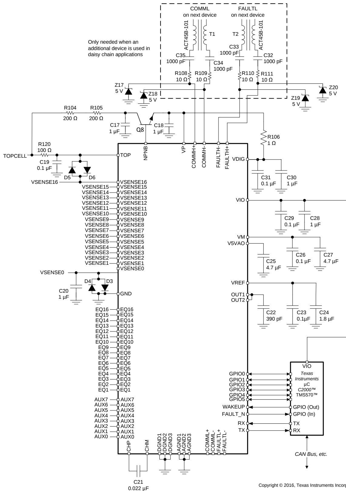
Figure 36. Main Device
