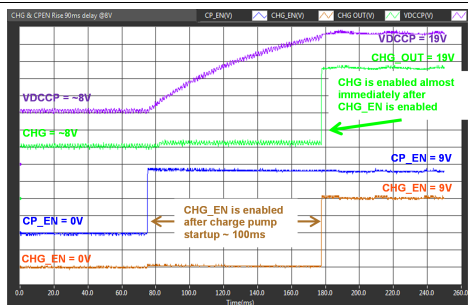
Figure 12. CHG_EN Switched On After Charger Pump Turns On and Is Stable
