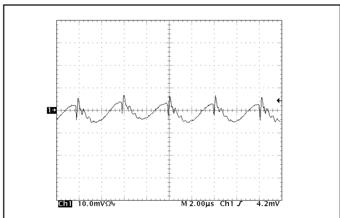
Figure 15: Input reflected ripple current, i_s , through a 10 µH source inductor, using a 47 µF electrolytic input capacitor (50 mA/div). See Figure 13.
