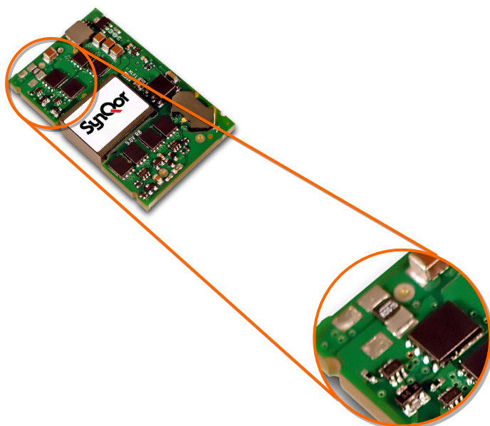
Figure G: Location of Sense Resistor
