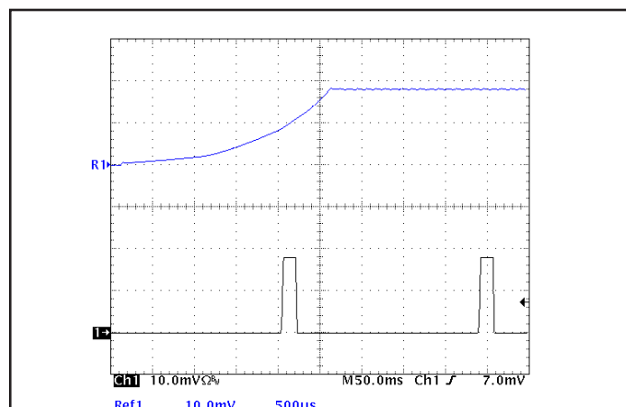
Figure 18: Load current (50 A/div) as a function of time when the converter attempts to turn on into a 1 mΩ short circuit. Top trace (500 µs/div) is an expansion of the on-time portion of the bottom trace.
