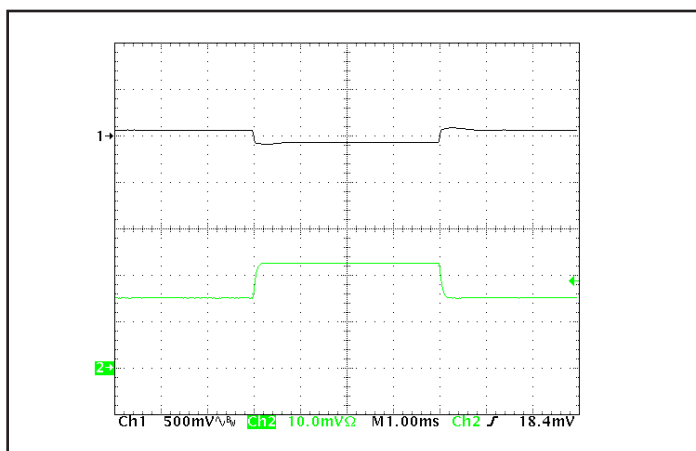
Figure 11: Output voltage response to step-change in load current (50%-75%-50% of I_{out(max)} ; dI/dt = 0.1 \text{ A}/\mu\text{s} ). Load cap: 15 \mu\text{F} tantalum cap and 1 \mu\text{F} ceramic cap. Ch 1: Vout (500 mV/div), Ch 2: Iout (20 A/div).
