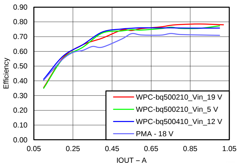
Figure 6. System Efficiency versus Output Current
