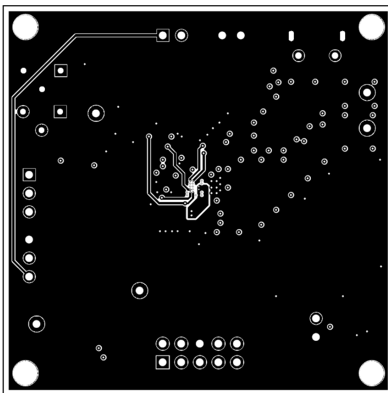
Figure 16. bq51221EVM-520 Layer 4
