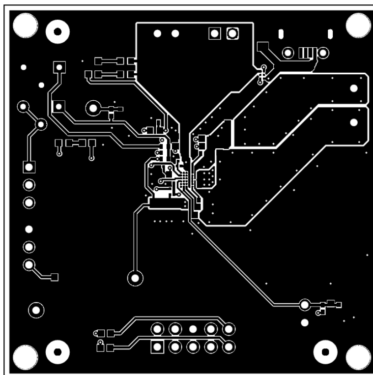
Figure 13. bq51221EVM-520 Layer 1
