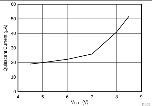
Figure 2. Quiescent Current as a Function of Output Voltage
