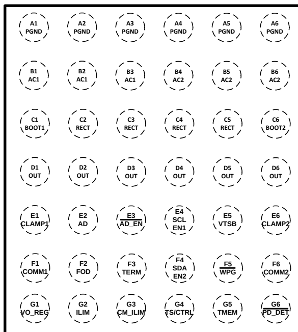
Pin Functions
