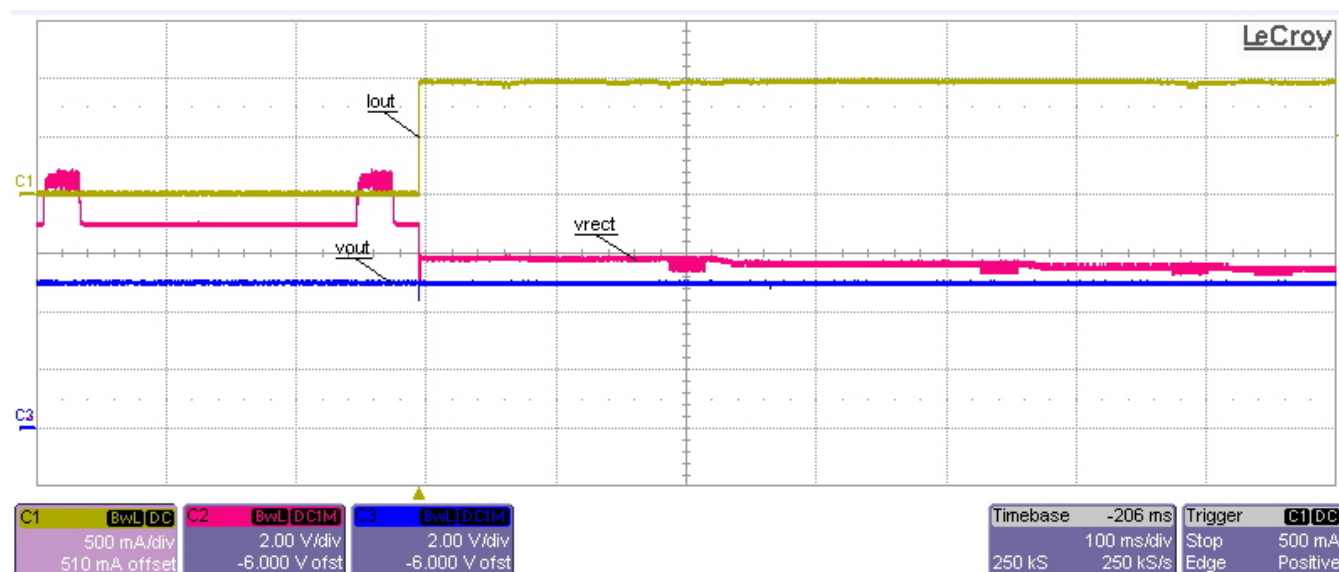
Figure 3. Load Step, 0 mA to 500 mA
