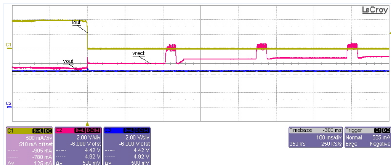
Figure 4. Load Dump, 500 mA to 0 mA
