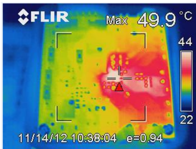
Figure 7. Thermal Image
