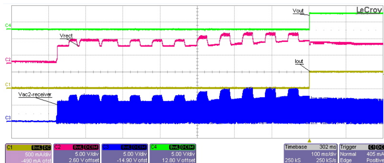
Figure 5. Start-Up
