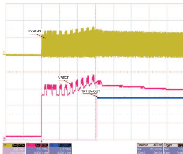
Figure 6. Start-Up
