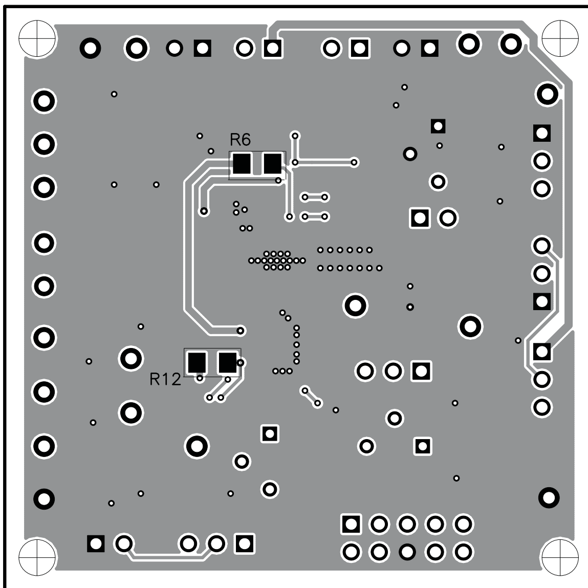
Figure 14. Bottom Assembly
