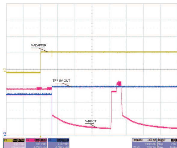
Figure 5. V-Adapter Input
