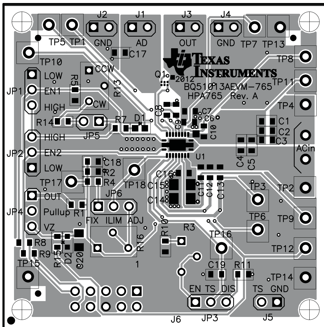
Figure 11. Top Assembly
