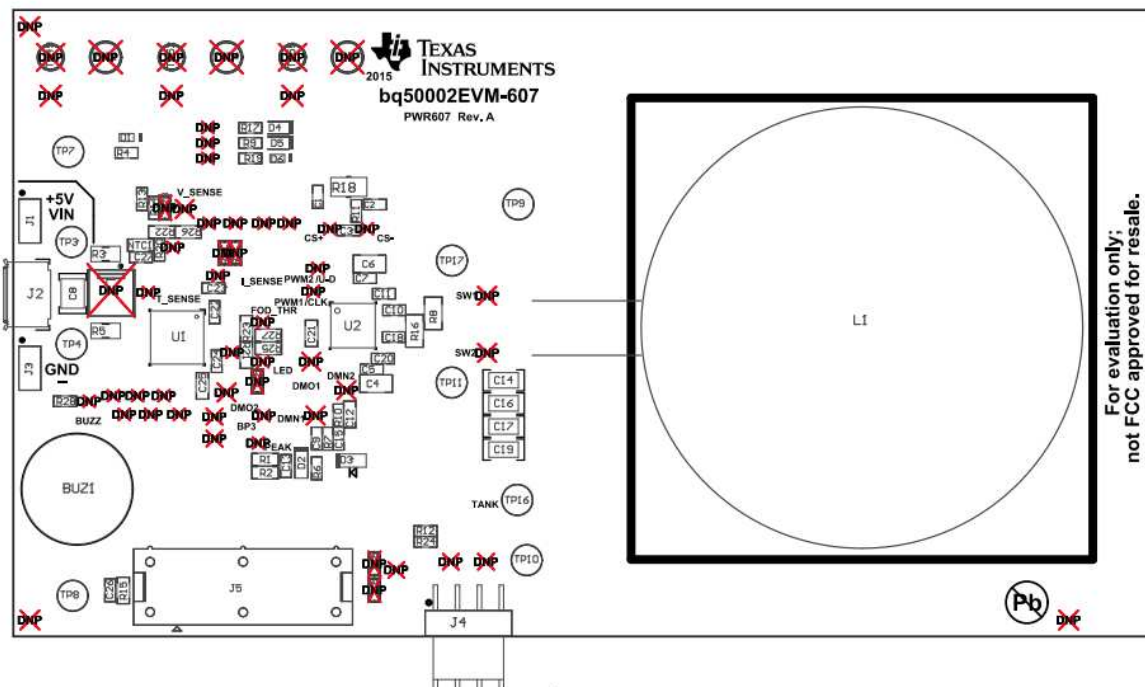
Figure 8. Assembly Top
