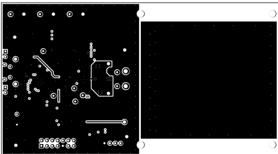
Figure 11. Bottom Layer
