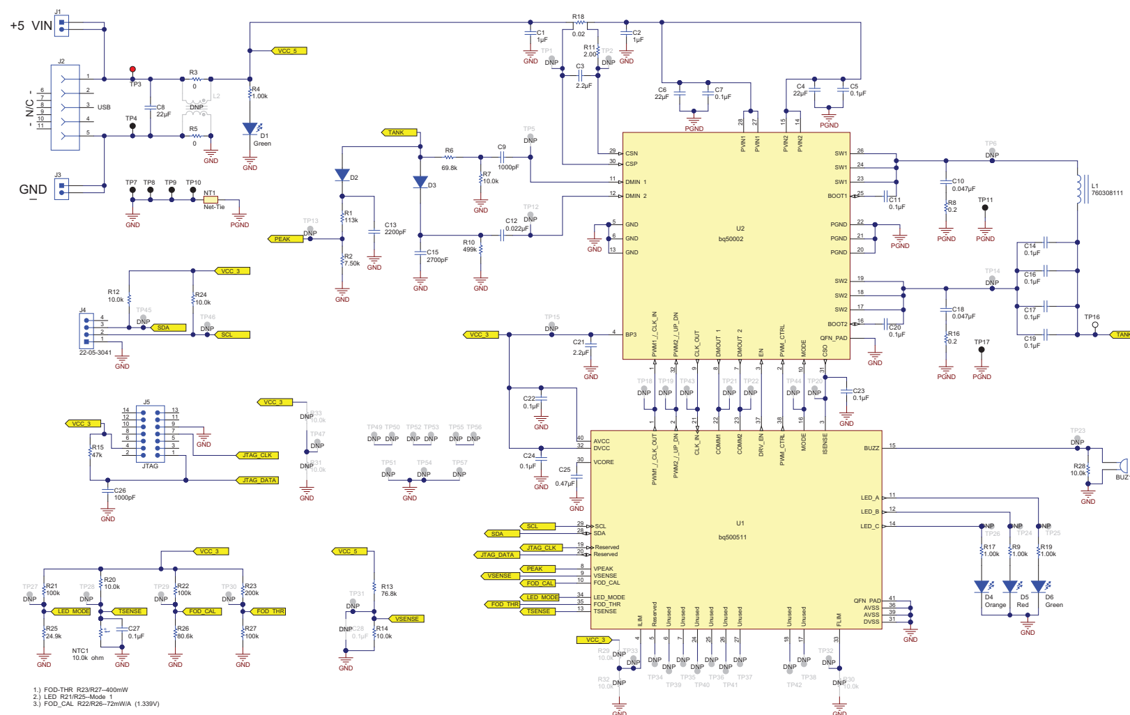
Figure 1. bq50002EVM-607 Schematic
