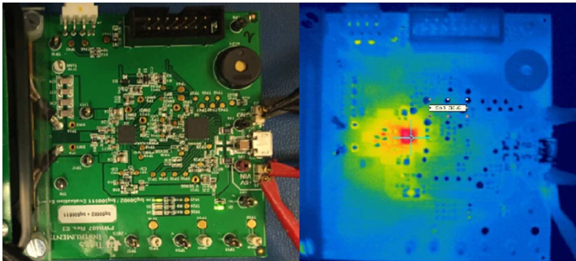
Figure 7. Thermal Performance
