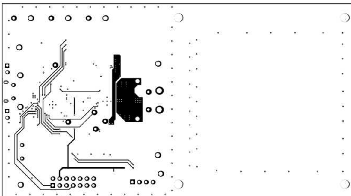
Figure 10. Inner Layer 2
