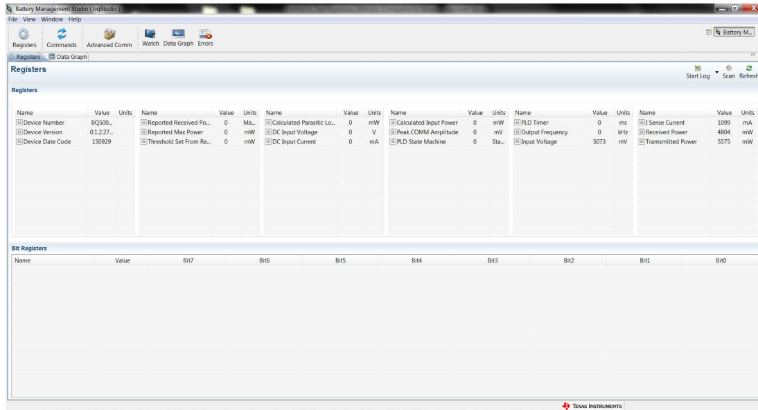
Figure 3. bqStudio Window
