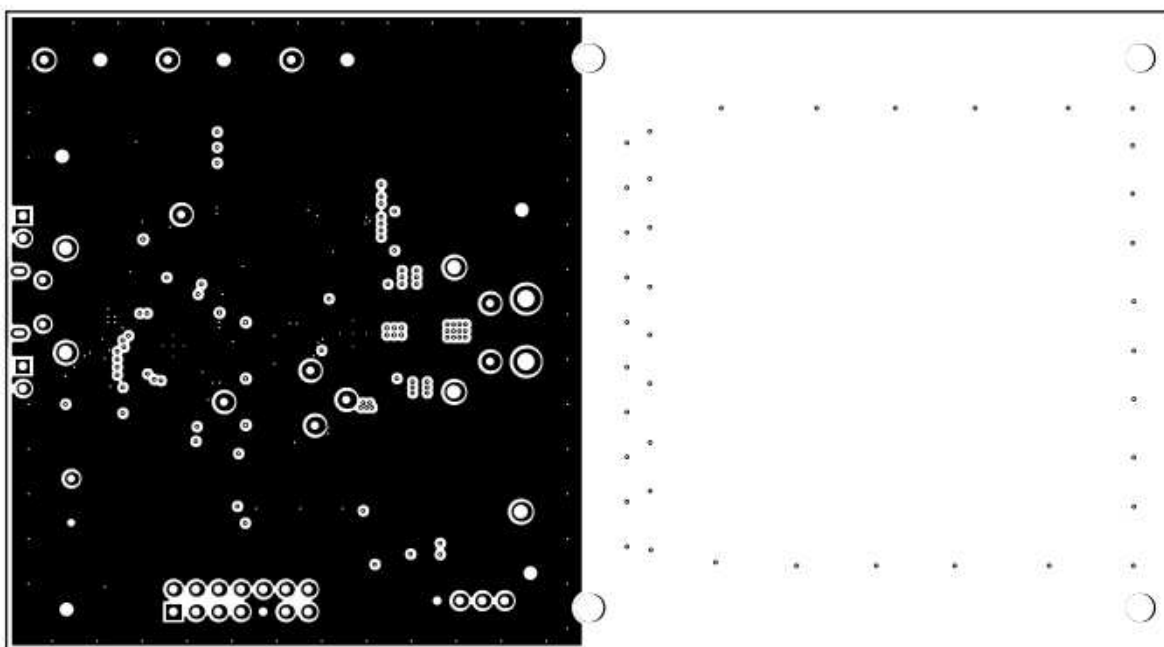
Figure 9. Inner Layer 1
