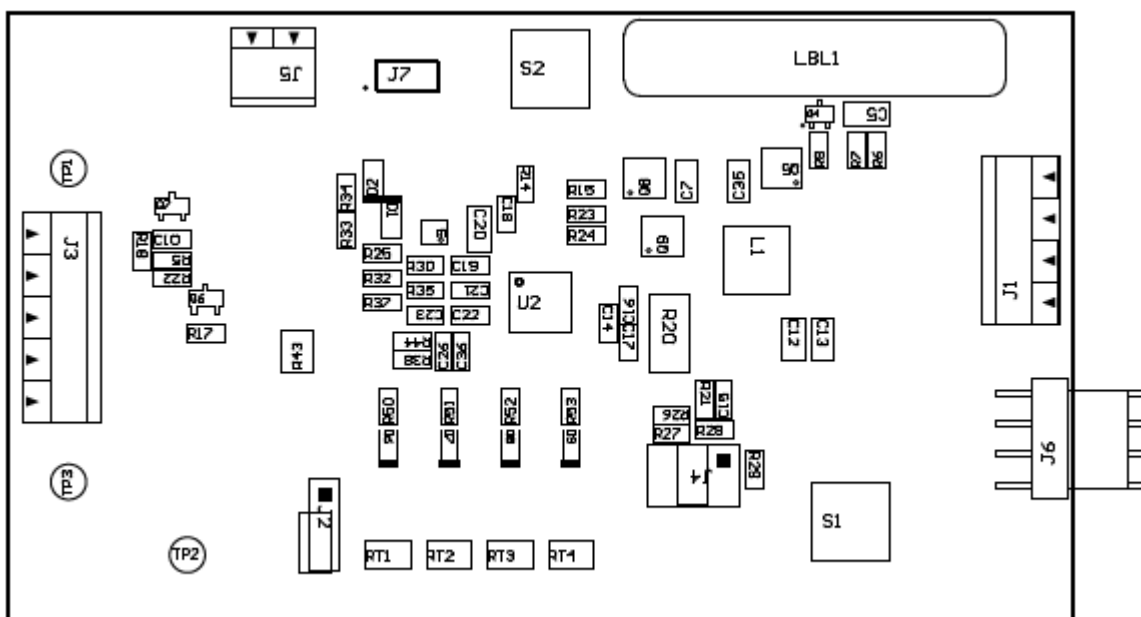
Figure 11. Top Assembly
