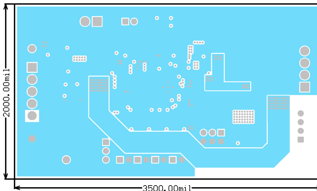
Figure 14. Internal Layer 1
