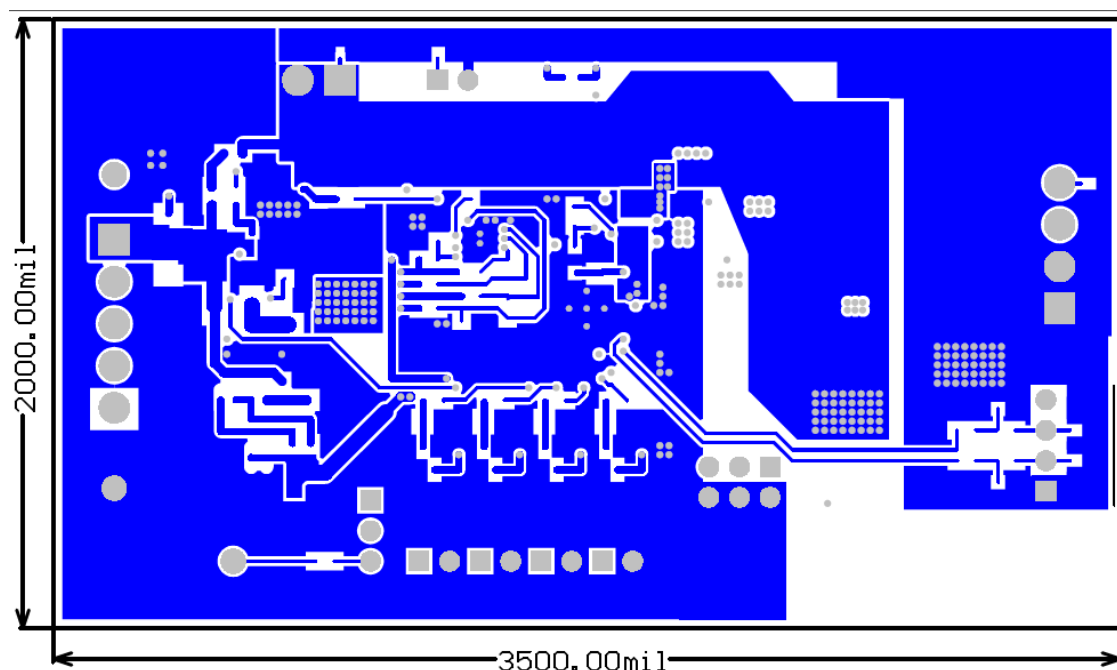
Figure 16. Bottom Layer
