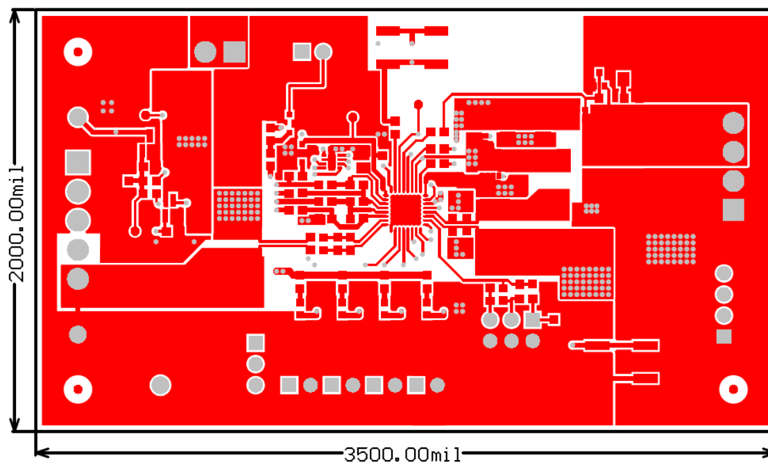
Figure 13. Top Layer
