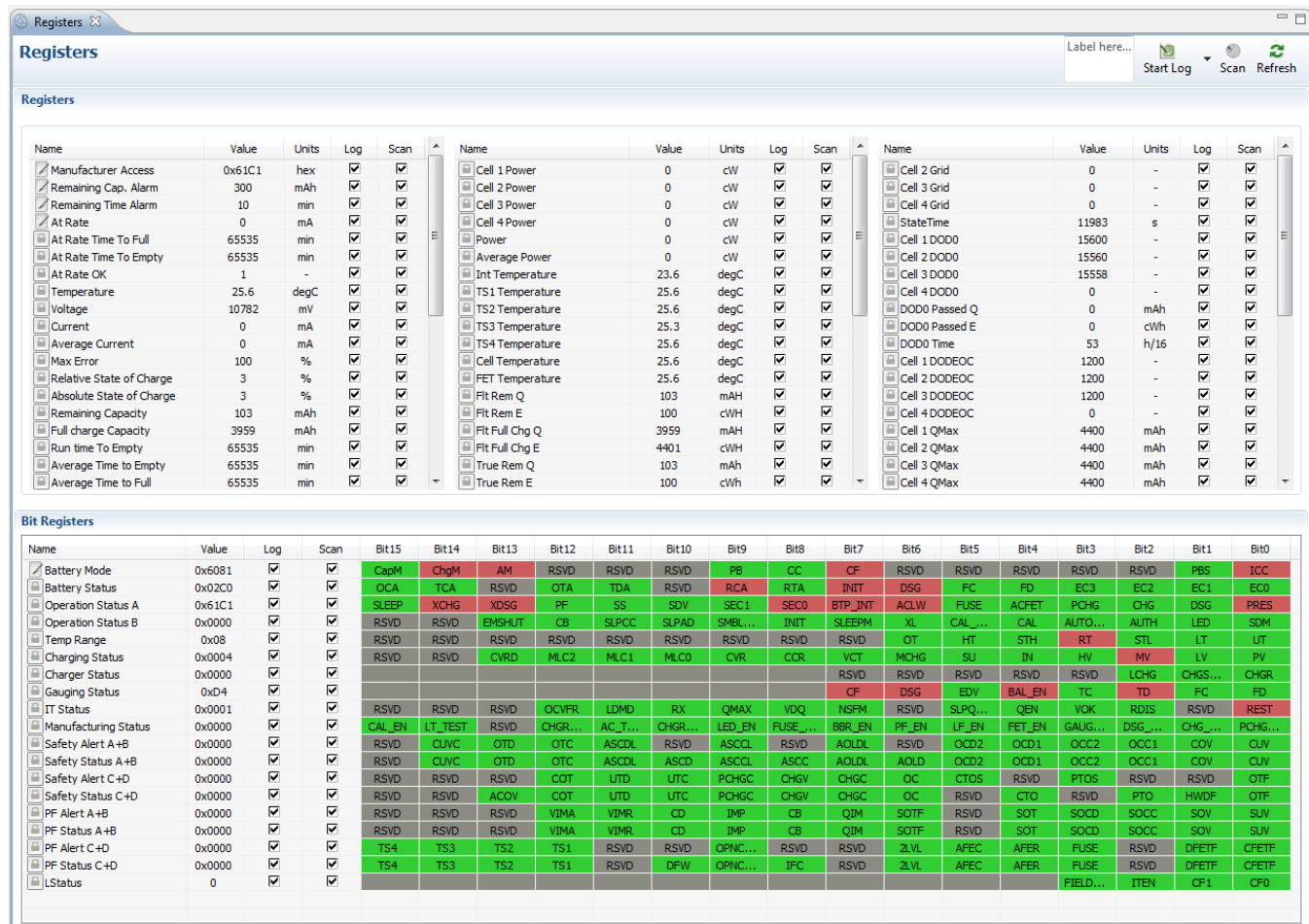
Figure 2. Registers Screen
