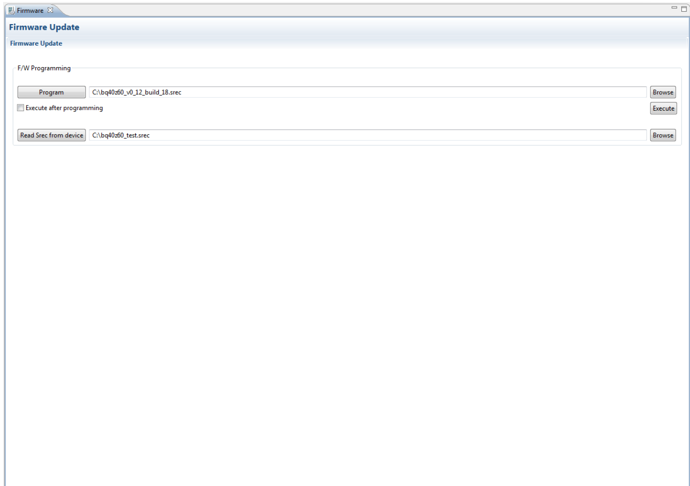
Figure 6. Firmware Screen
