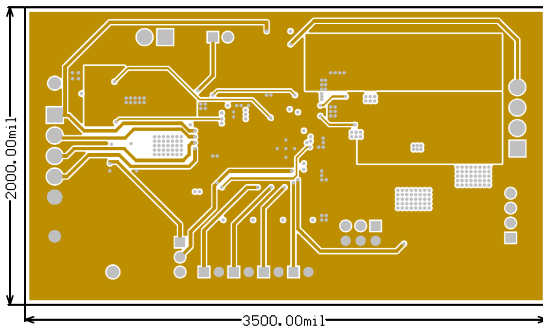
Figure 15. Internal Layer 2
