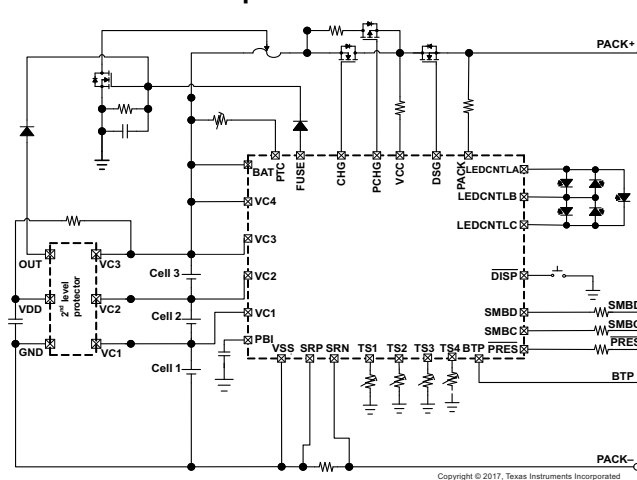
Simplified Schematic
