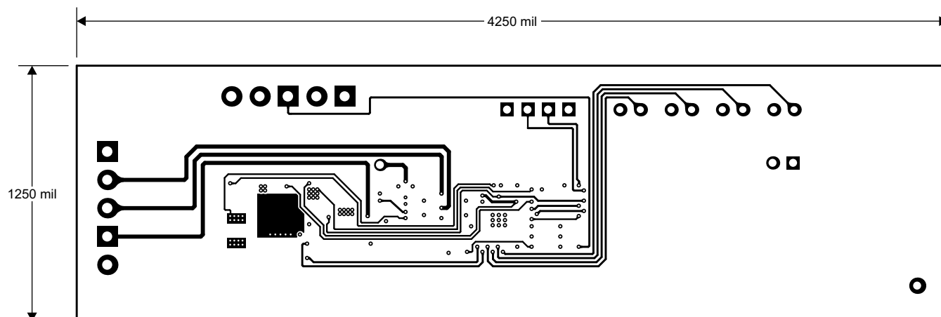
Figure 15. Inner Layer 2
