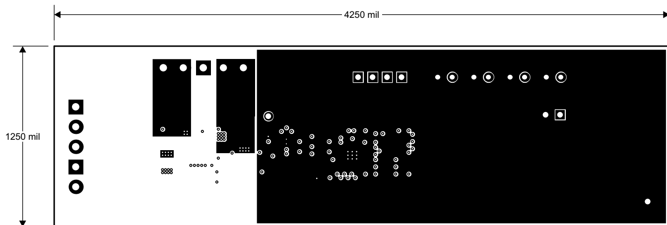
Figure 14. Inner Layer 1
