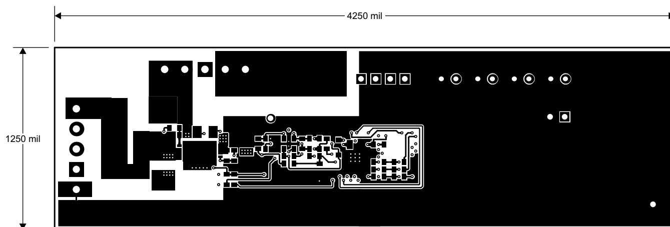
Figure 16. Bottom Layer
