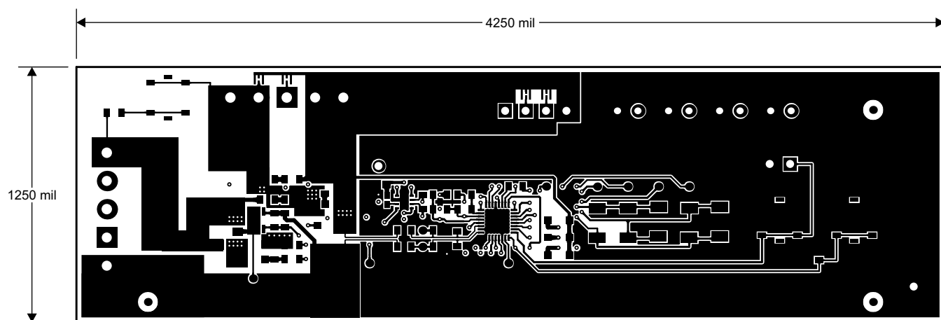
Figure 13. Top Layer
