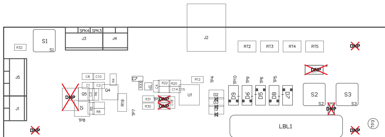
Figure 11. Top Assembly
