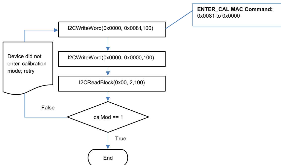
Figure 3-1. Enter CALIBRATION Mode Flow
