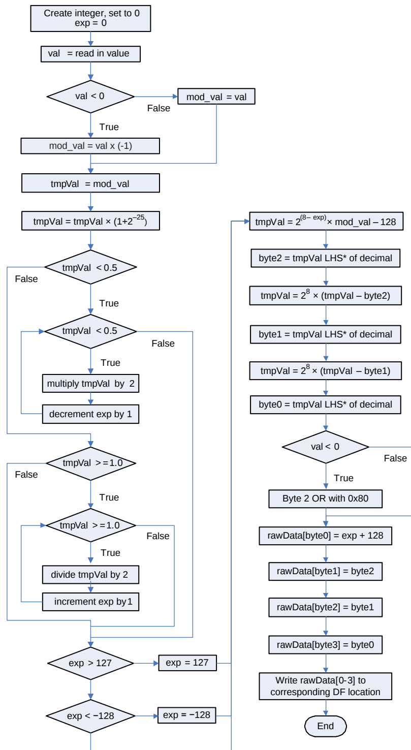
Figure 3-8. Floating Point Conversion Flow
