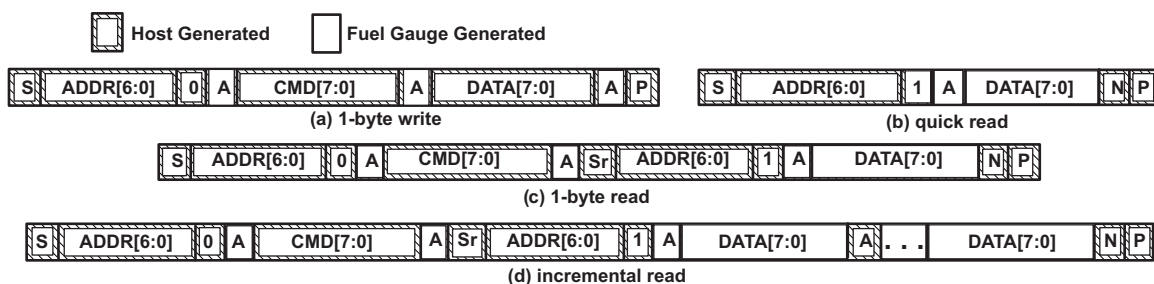
Figure 14-1. Supported I 2 C Formats
