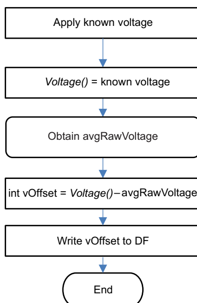
Figure 3-2. Voltage Calibration Flow
