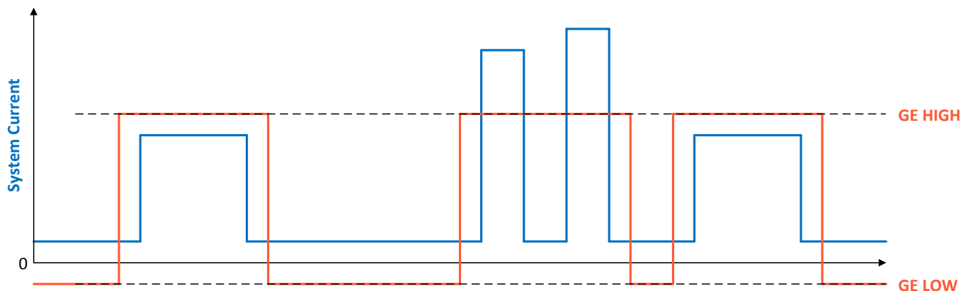
Figure 6-1. System Current Profile Example
