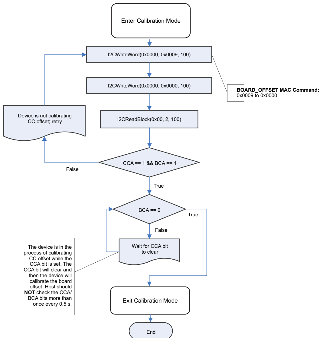
Figure 3-4. Board Offset Flow
