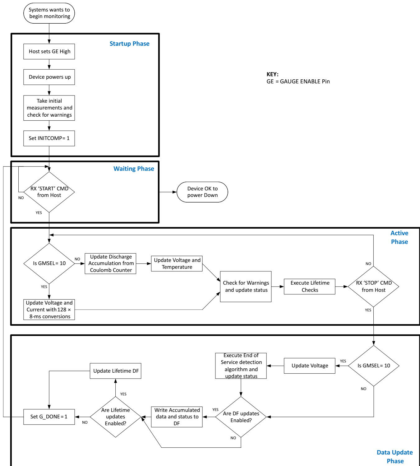
Figure 6-2. Operational Flow
