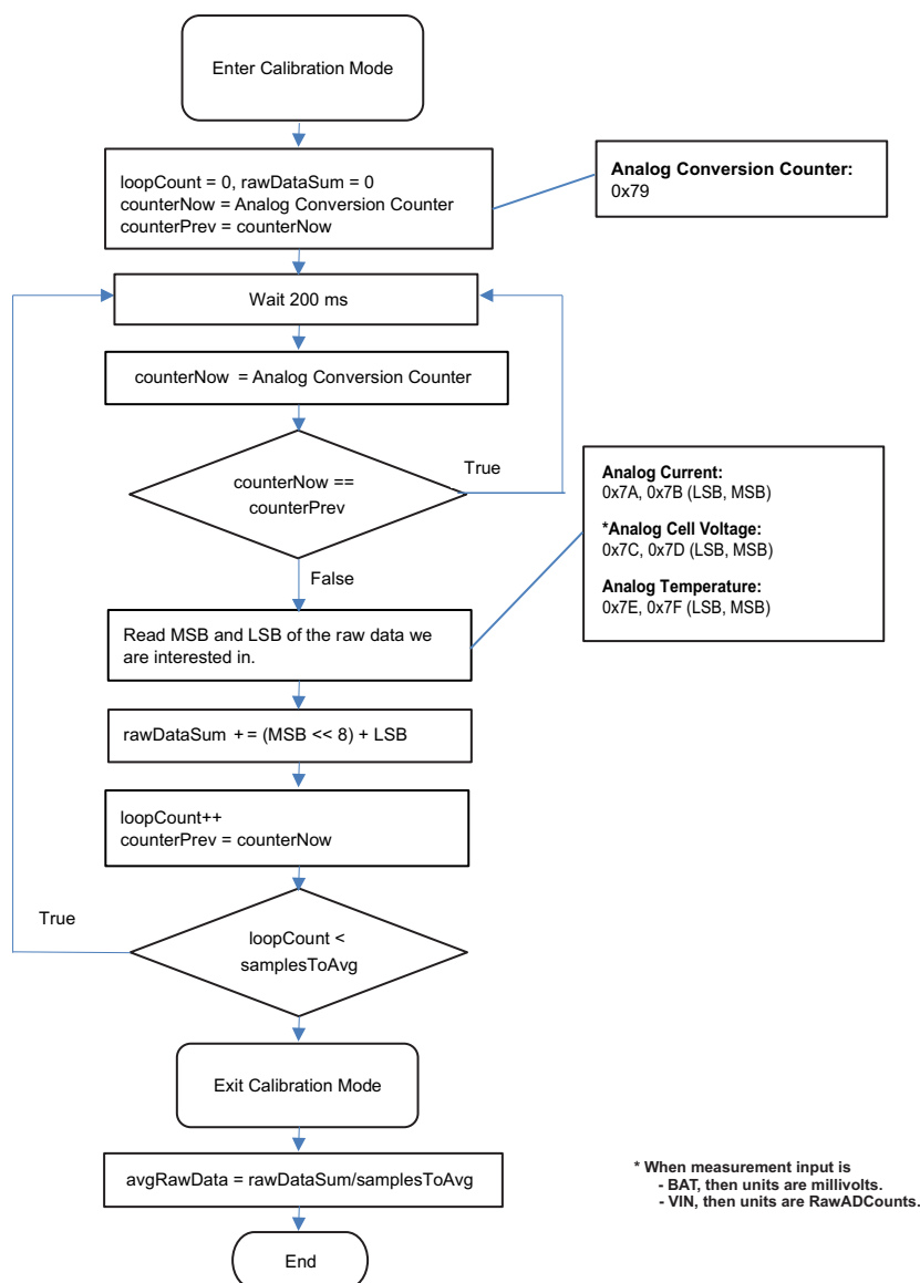
Figure 3-5. Obtain Raw Calibration Data Flow
