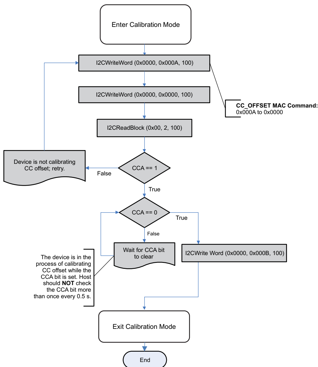
Figure 3-3. CC Offset Flow
