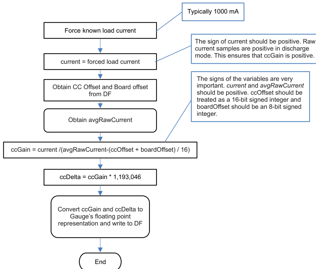
Figure 3-6. Current Calibration Flow
