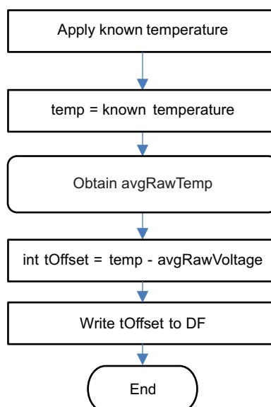
Figure 3-7. Temperature Calibration Flow
