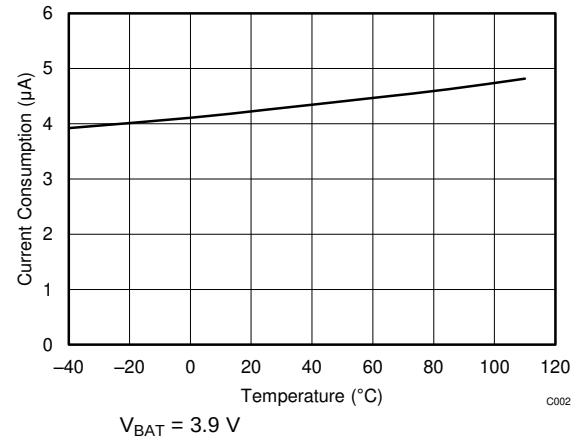
Figure 2. 3.9-V I_{BAT} Versus Temperature
