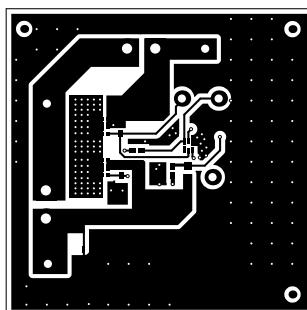
Figure 3. Top Layer
