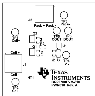
Figure 2. Top Assembly
