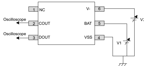
Figure 24. Test Circuit 5
