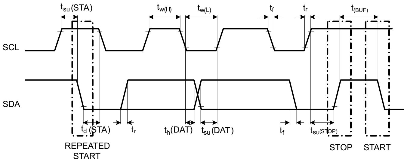
Figure 1. Timing
