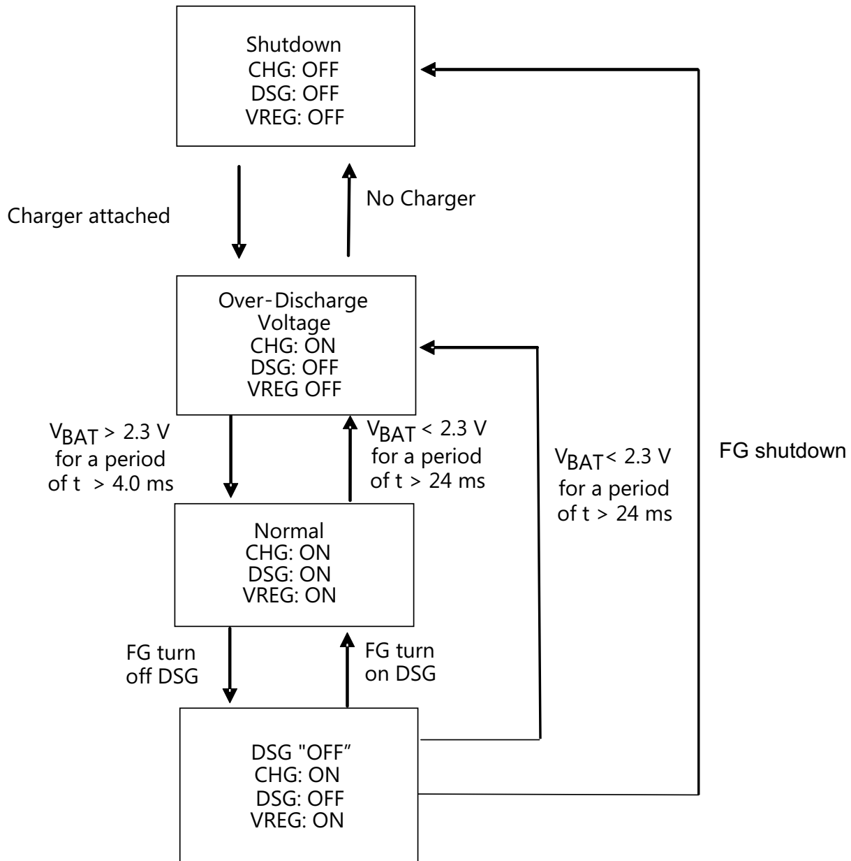
Figure 4. Shutdown Operation
