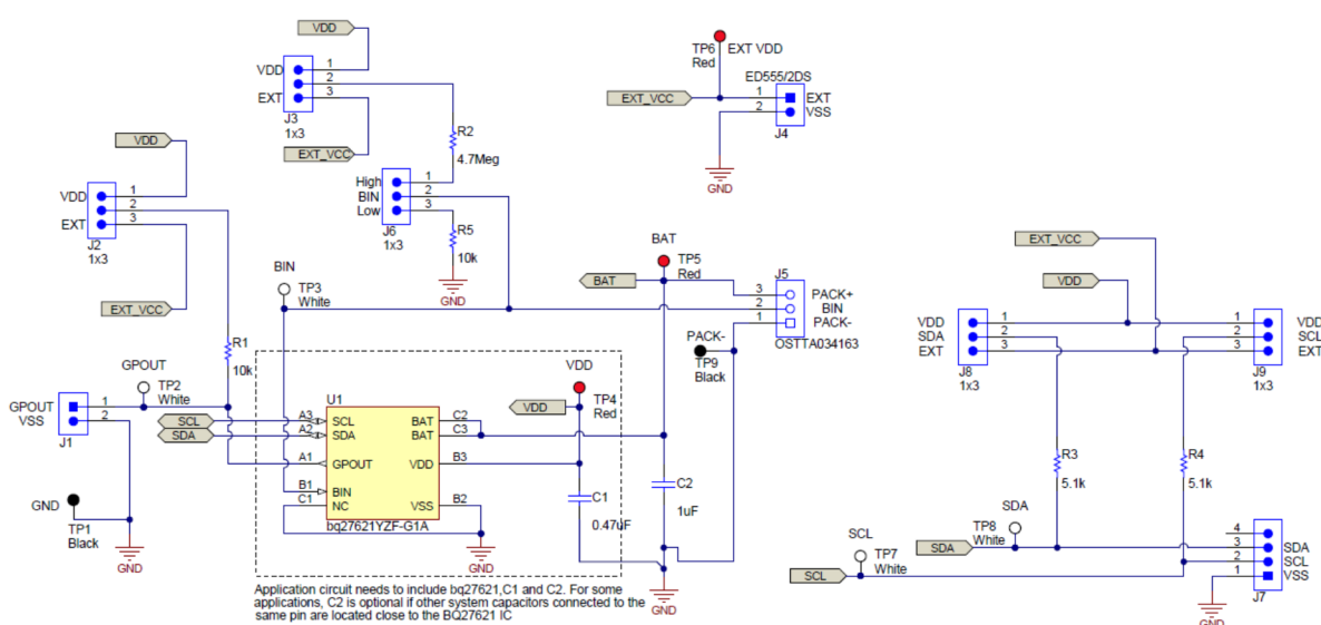
Figure 9. Reference (EVM) Schematic
