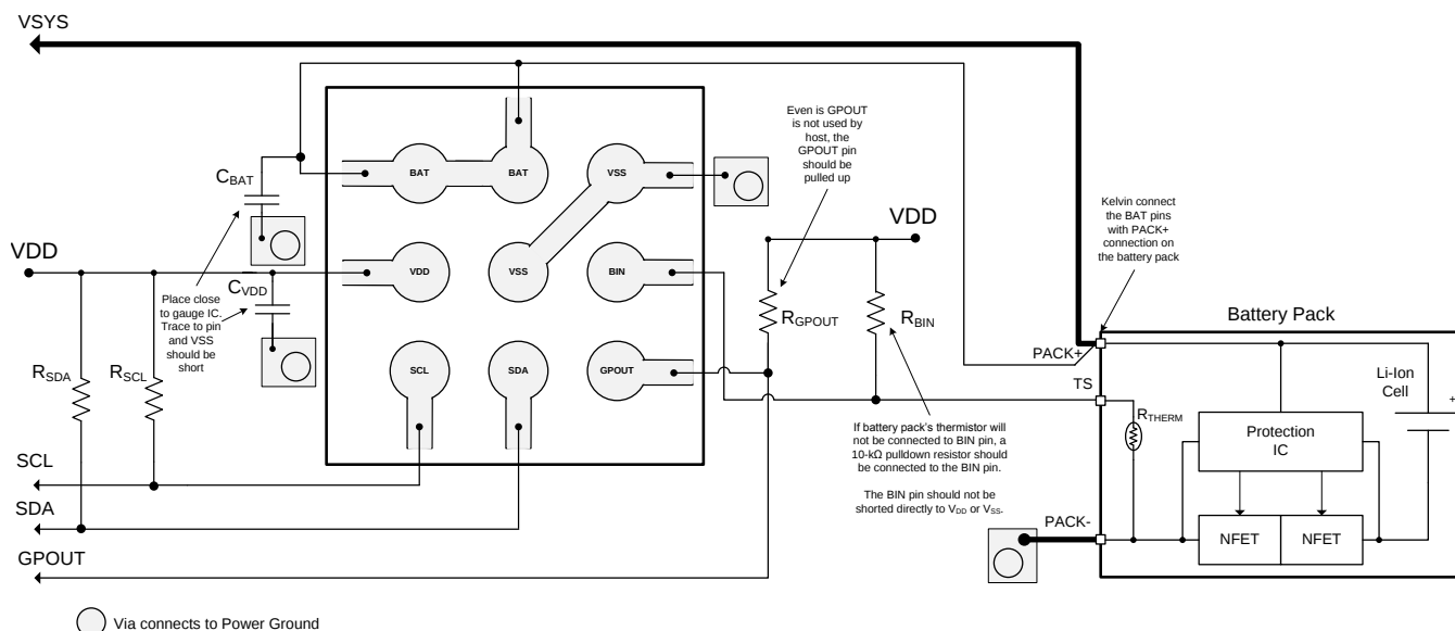
Figure 13. Layout Example
