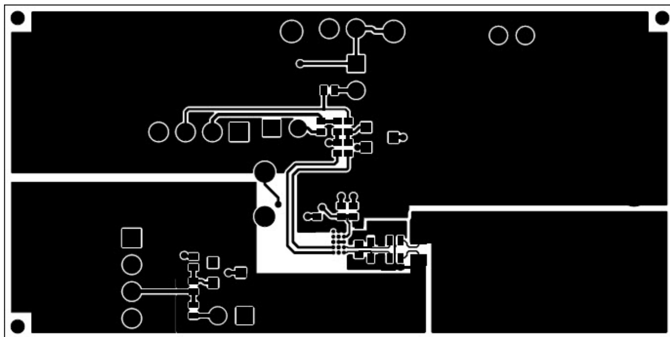
Figure 3. Top Layer
