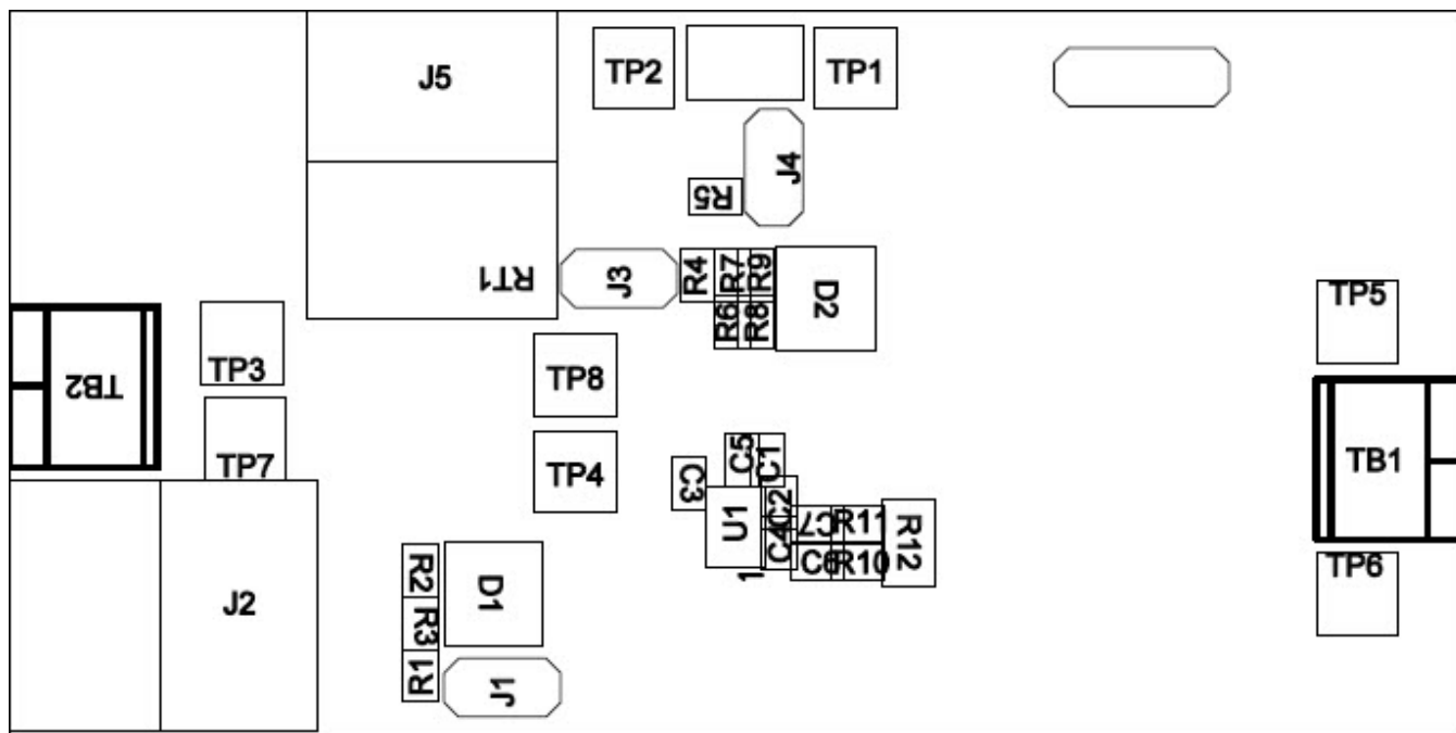
Figure 2. Top Assembly
