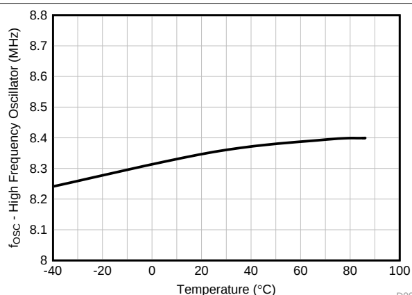
Figure 14. High-Frequency Oscillator Frequency vs. Temperature
