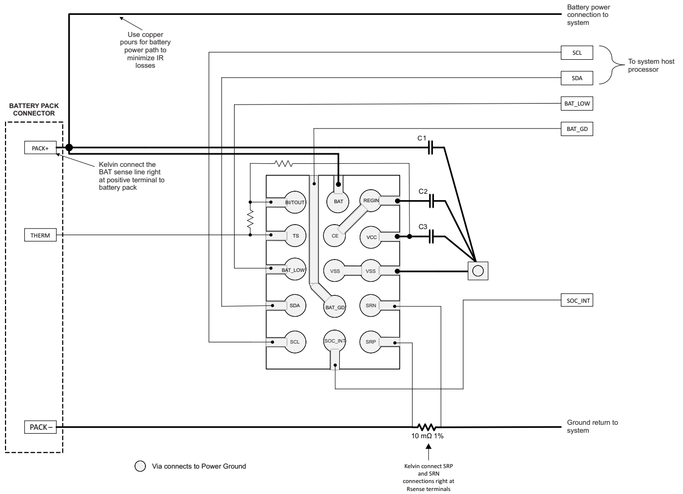
Figure 17. Layout Recommendation
