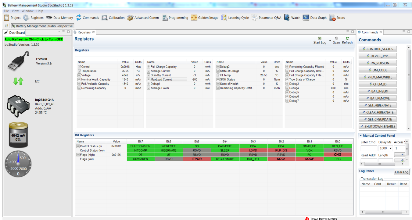
Figure 8. Registers Screen
