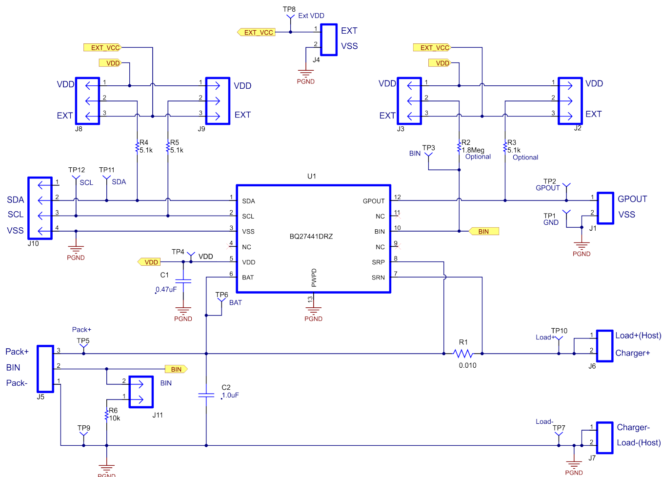
Figure 6. bq27441EVM Schematic
