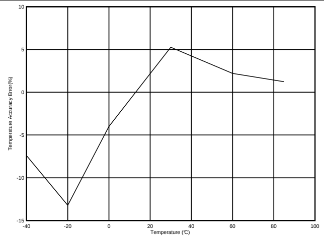
Figure 8. Temperature Accuracy
