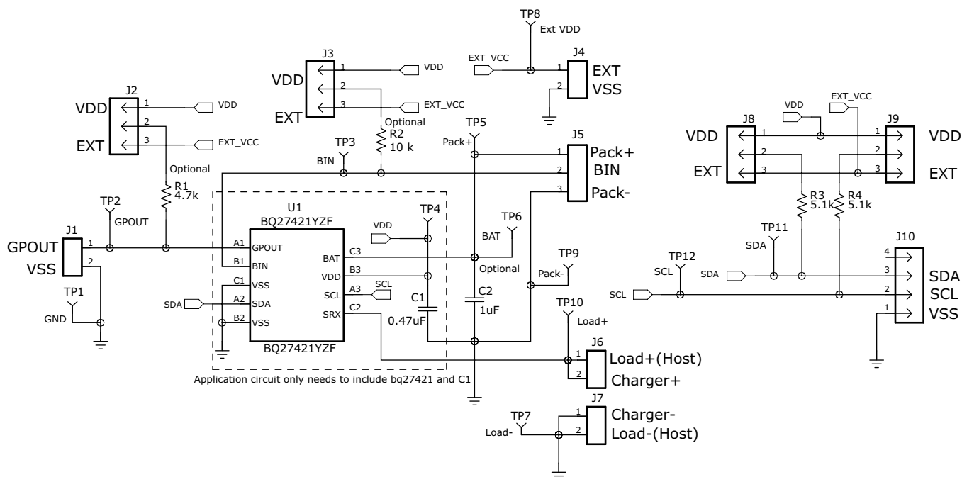
Figure 6. bq27421EVM Schematic
