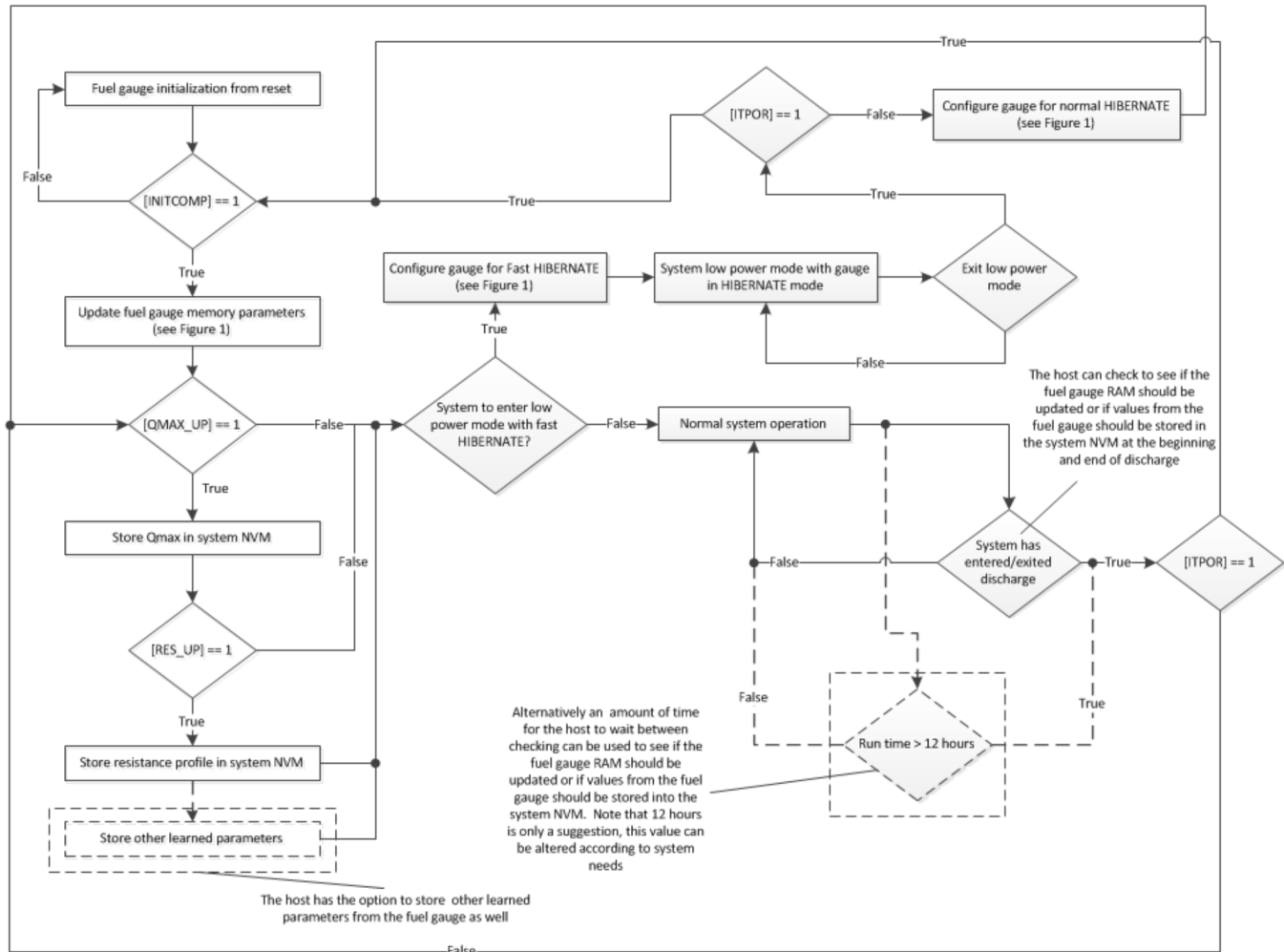
Figure 4. Recommended System Operation Flowchart
