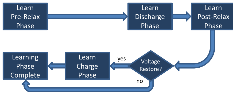
Figure 1-5. State Diagram for LSM = 1
