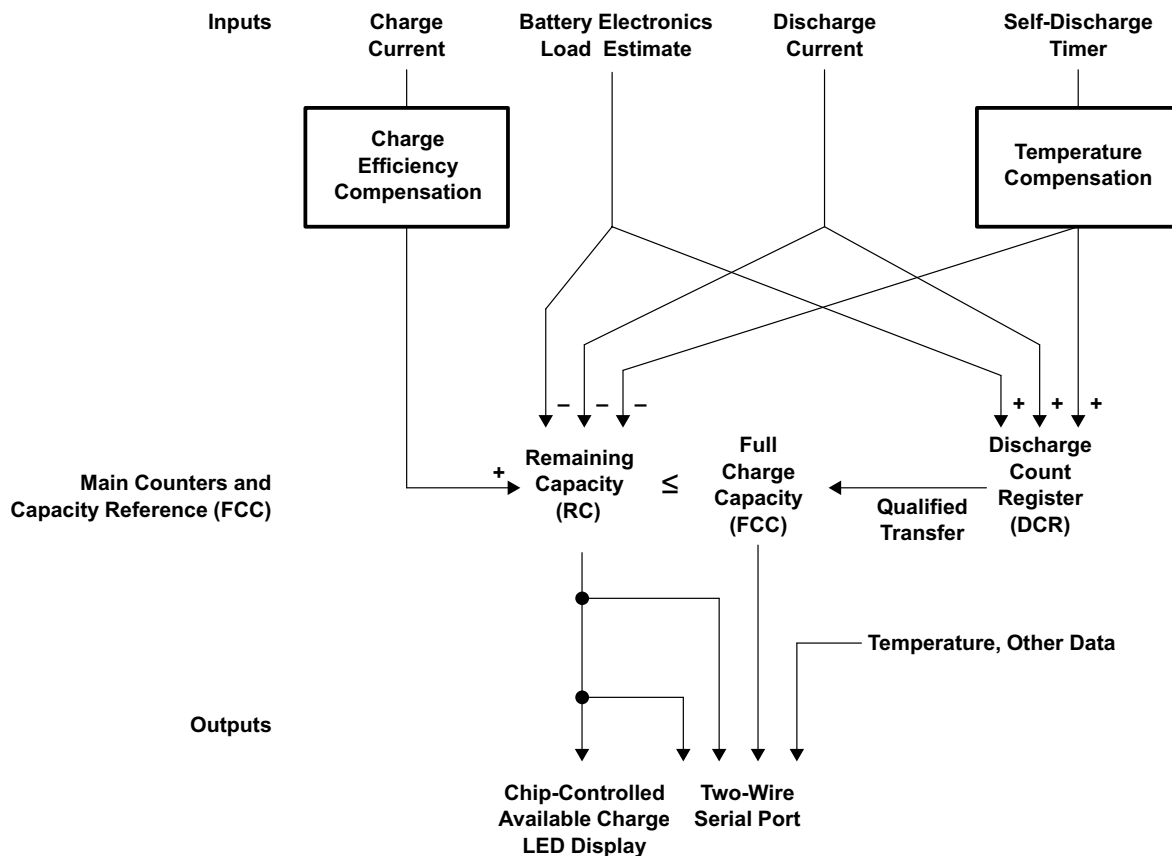
Figure 1-1. bq34210-Q1 CEDV Gas Gauging Operational Overview
