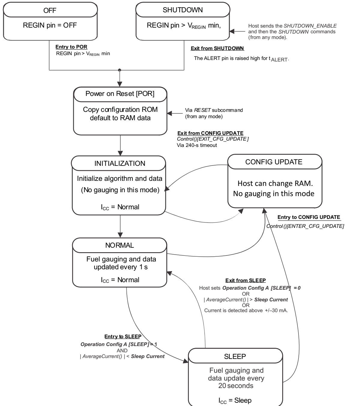
Figure 2-1. Power Mode Diagram for System Shutdown
