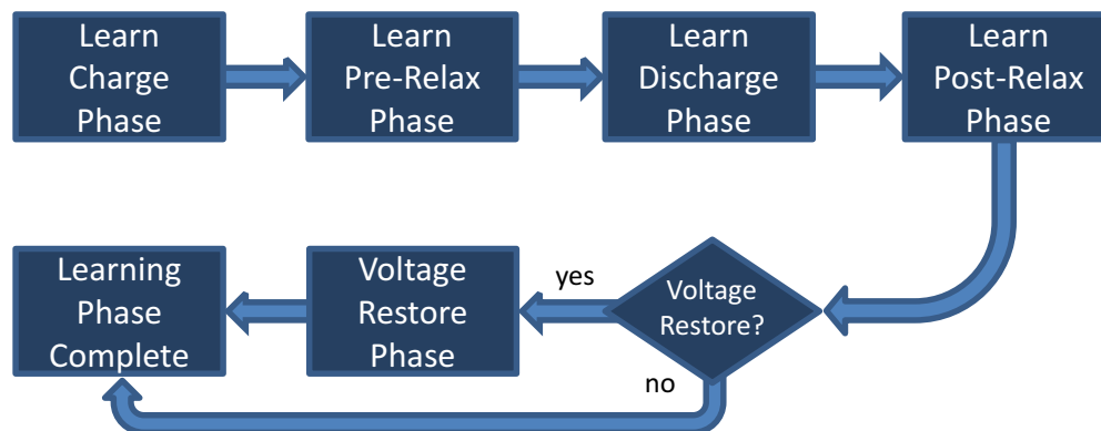
Figure 1-4. State Diagram for LSM = 0
