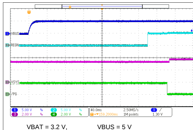
Figure 50. Power Up with Charge Disabled
