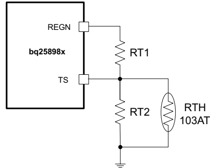
Figure 16. TS Resistor Network
