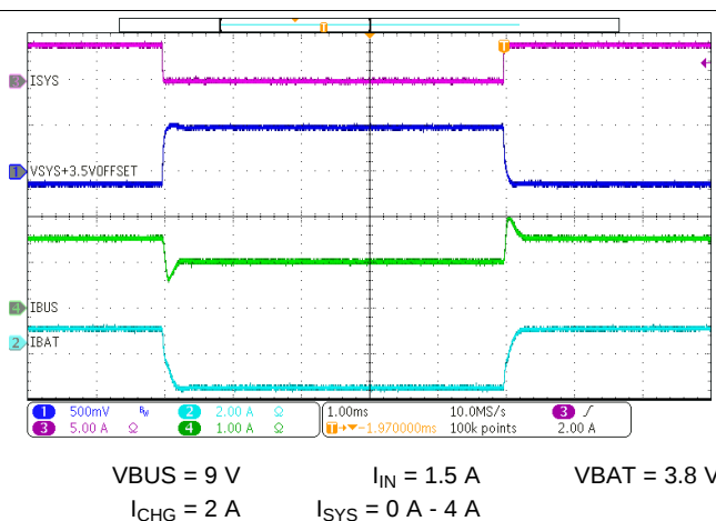
Figure 55. Load Transient During Supplement Mode
