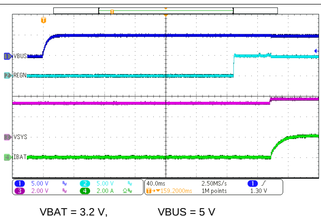
Figure 51. Power Up with Charge Enabled
