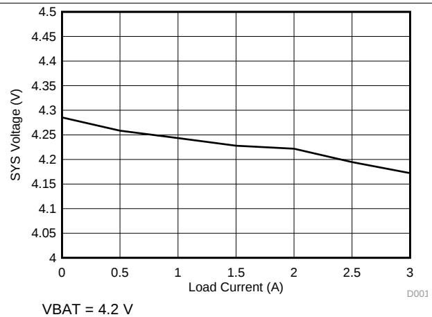
Figure 6. SYS Voltage Regulation vs System Load Current
