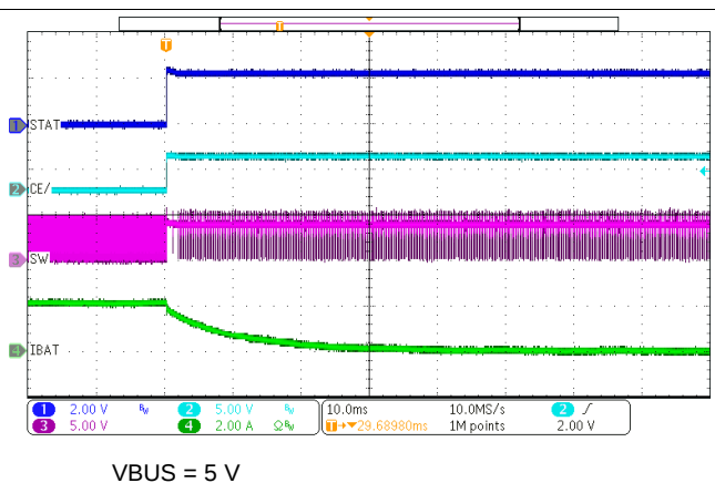
Figure 53. Charge Disable
