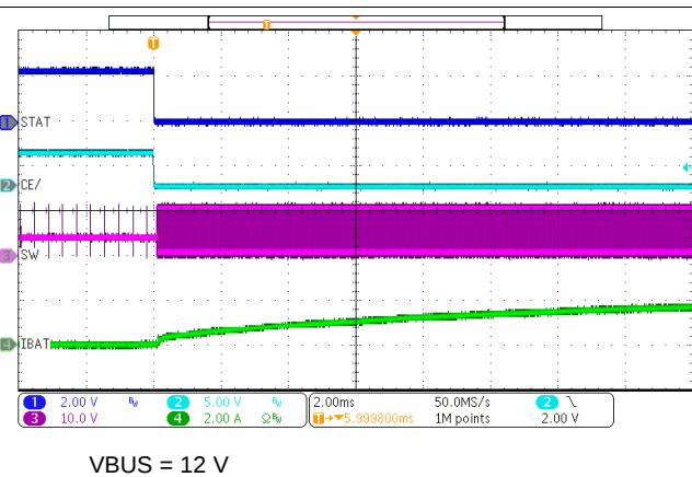
Figure 61. Charge Enable
