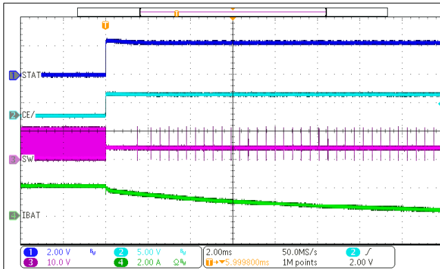
Figure 62. Charge Disable
