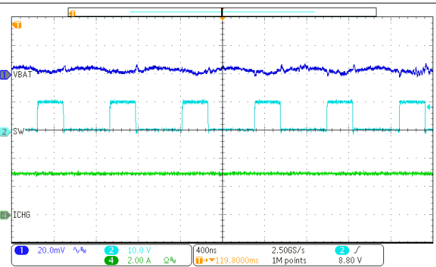
Figure 63. PWM Switching Waveform
