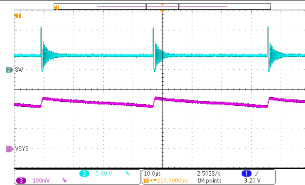
Figure 62. Charge Disable
