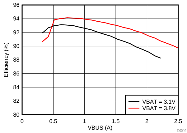
Figure 3. Boost Mode Efficiency vs VBUS Load Current
