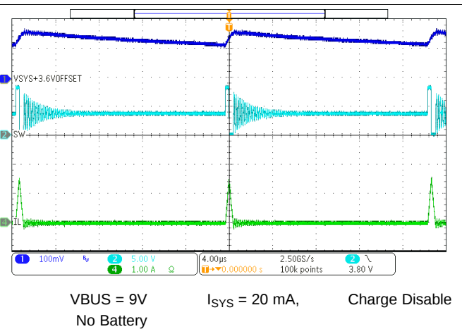
Figure 57. PFM Switching Waveform
