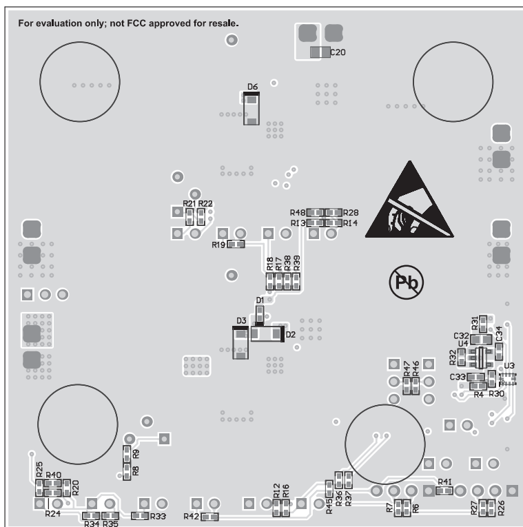
Figure 13. Top Layer
