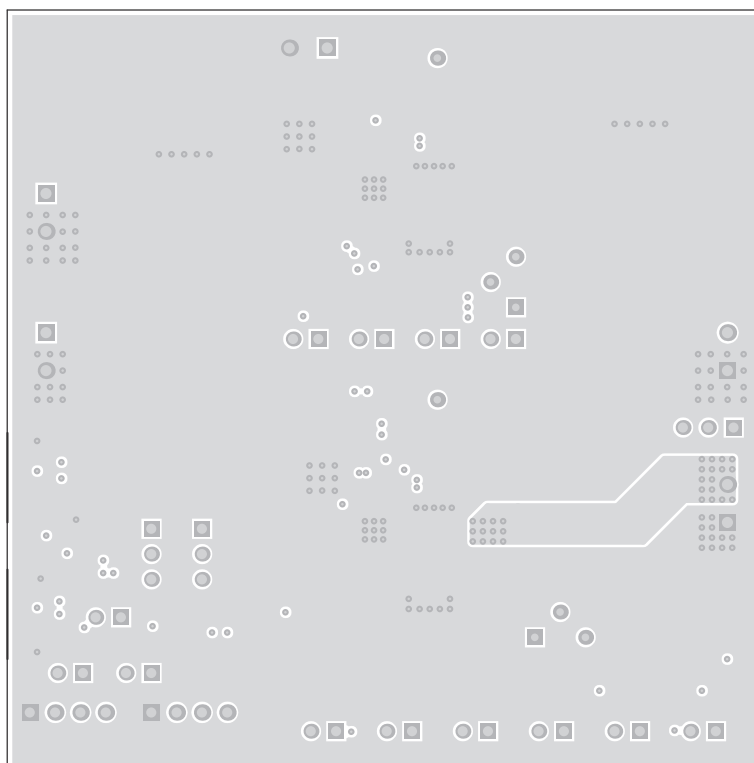
Figure 11. Internal Layer 1
