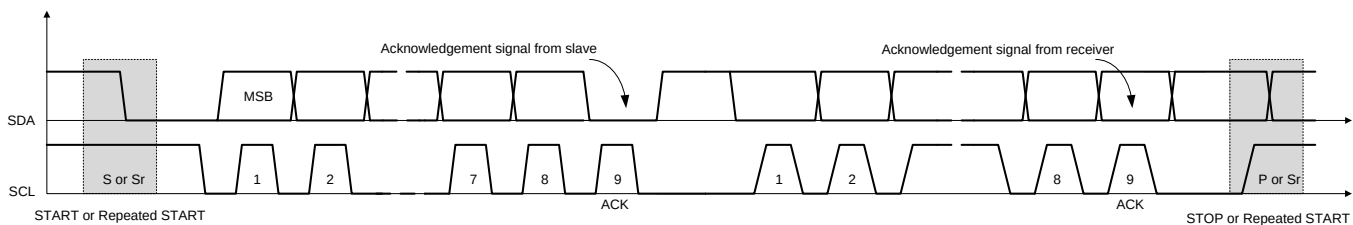
Figure 16. Data Transfer on the I²C Bus
