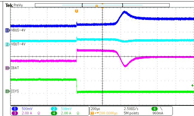
Figure 57. IBAT Regulation During Load Step Down
