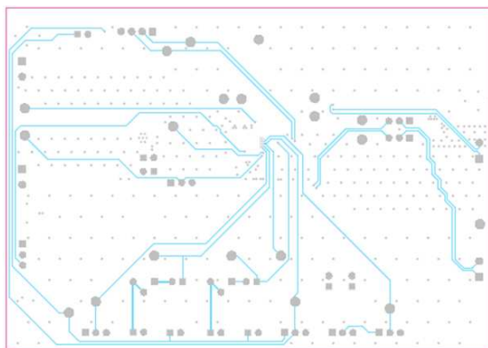
Figure 64. bq25872 Layout Diagram (Mid Layer 2)
