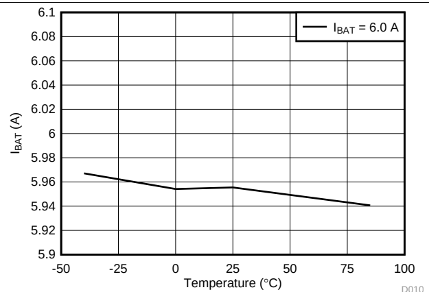
Figure 10. IBAT Regulation vs Temperature at 6 A
