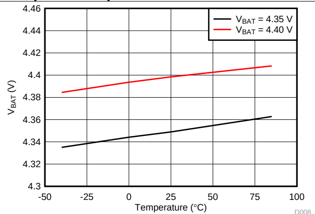
Figure 8. VBAT Regulation vs Temperature
