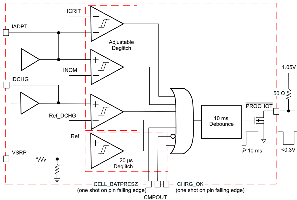
Figure 13. PROCHOT Profile
