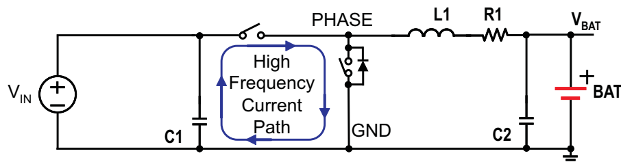
Figure 65. High Frequency Current Path
