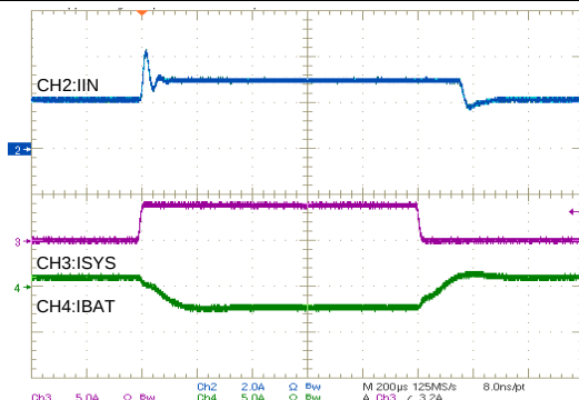
Figure 60. Input Current in Boost Mode
