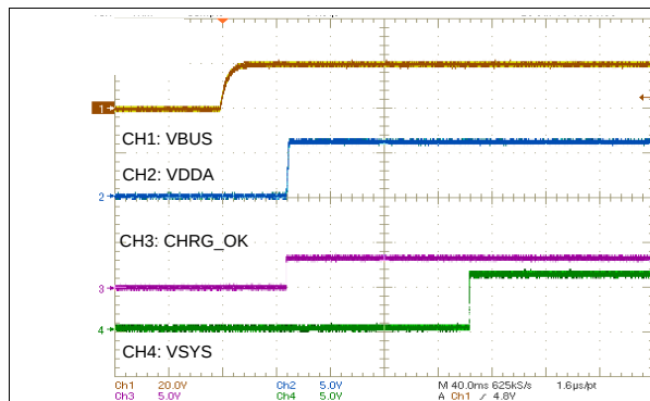
Figure 48. Power Up from 20 V
