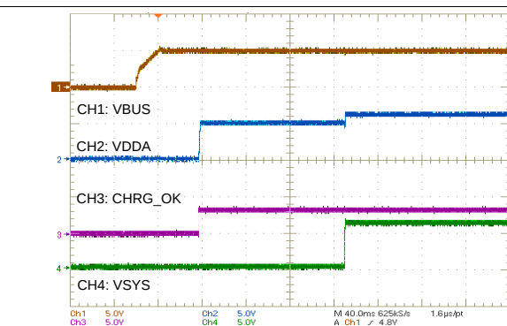
Figure 49. Power Up from 5 V
