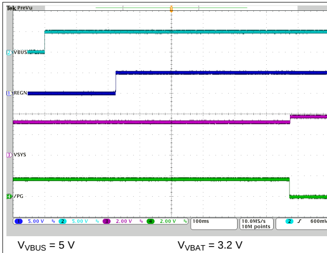
Figure 16. Power-Up with Charge Disabled
