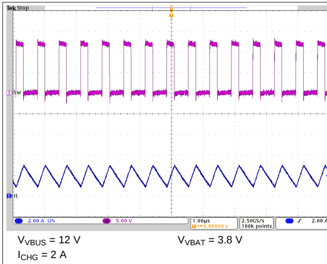
Figure 24. PWM Switching in Buck mode
