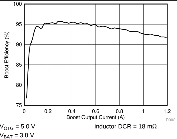
Figure 2. Efficiency vs. OTG Current
