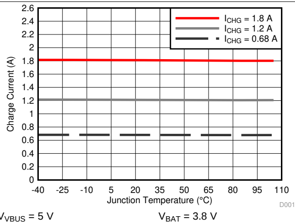
Figure 5. Charge Current vs. Junction Temperature
