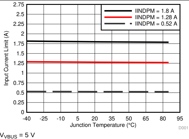
Figure 4. Input Current Limit vs. Junction Temperature
