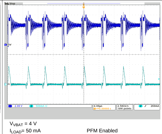
Figure 27. OTG Switching
