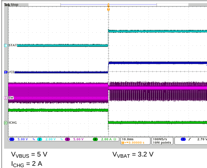
Figure 26. Charge Disable
