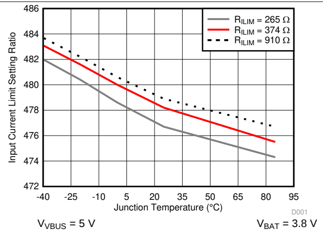
Figure 6. Input Current Limit Setting Ratio vs. Junction Temperature
