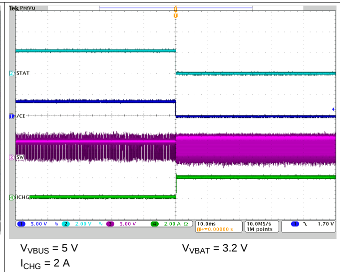
Figure 25. Charge Enable
