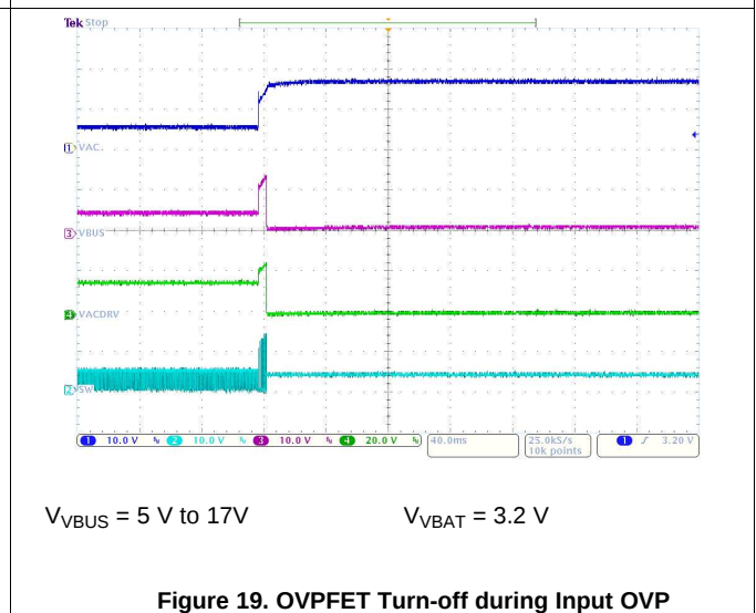
Figure 19. OVPFET Turn-off during Input OVP
