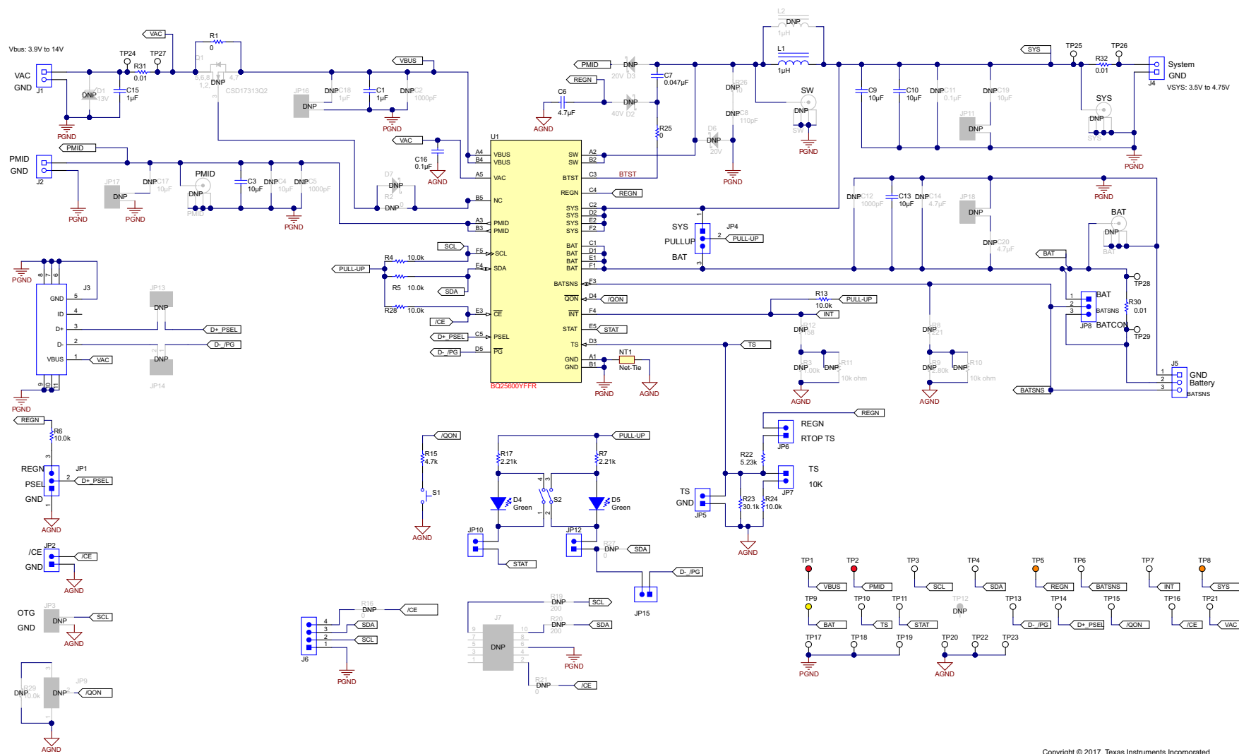
Figure 4. Schematic for bq25600 EVM
