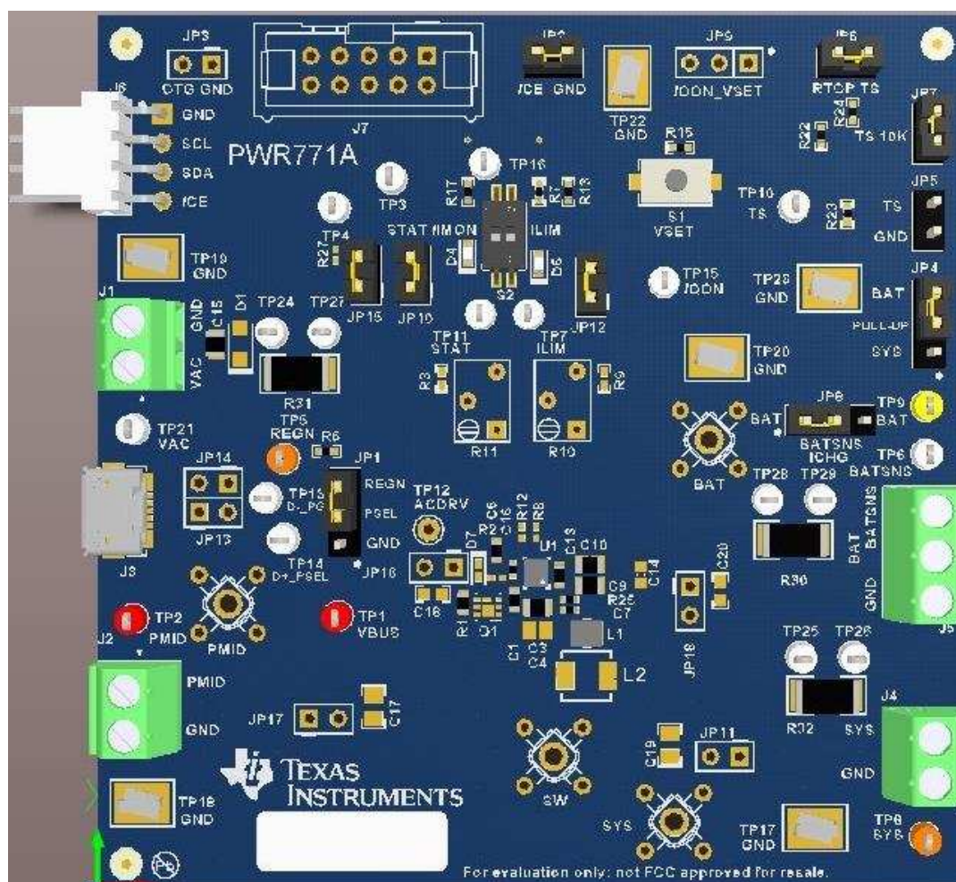
Figure 2. Original Test Setup for bq25600xEVM
