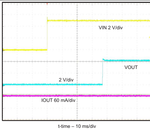
Figure 1. Power Up Timing
