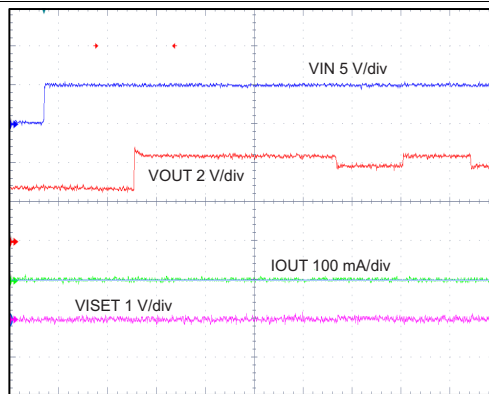
Figure 6. TS Enable and Disable
