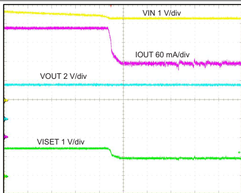
Figure 5. OVP from Normal Power-Up Operation
