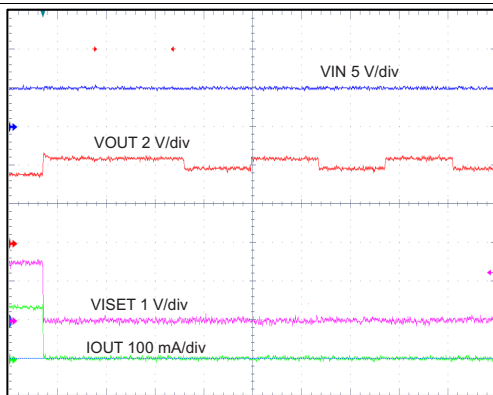
Figure 7. DPM-Adaptor Current Limits
