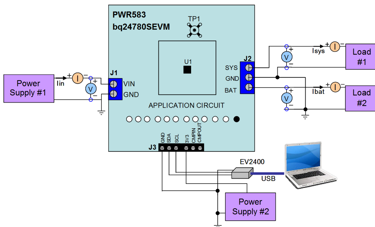
Figure 4. Test Setup for PWR583
