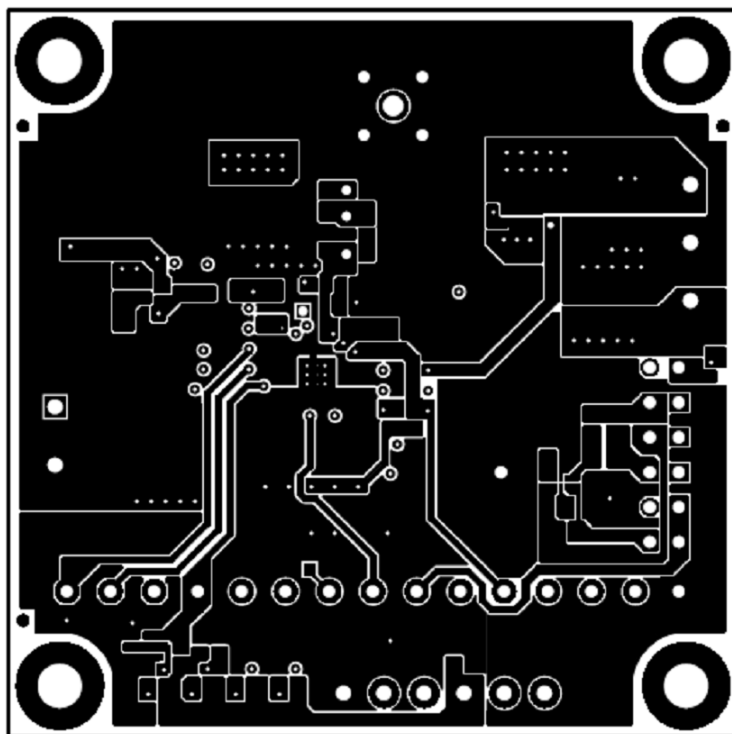
Figure 9. Bottom Layer
