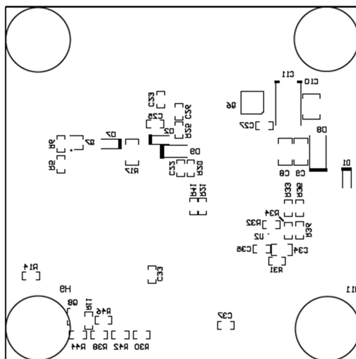
Figure 10. Bottom Assembly
