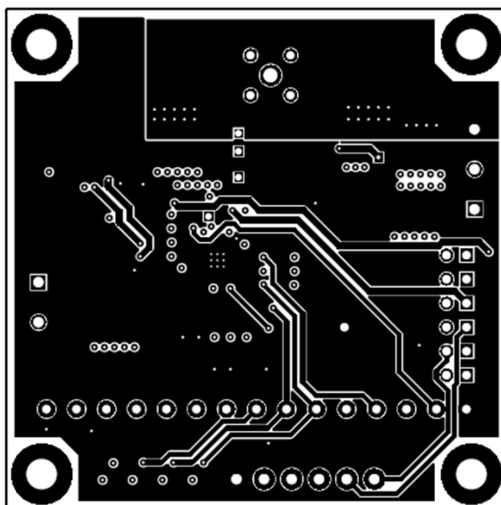
Figure 8. Mid-Layer 2
