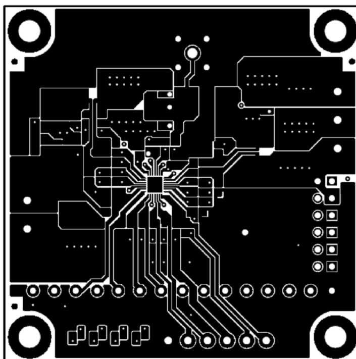
Figure 6. Top Layer
