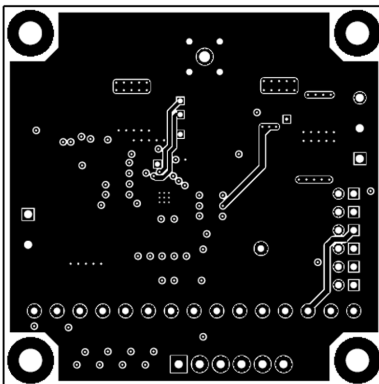
Figure 7. Mid-Layer 1
