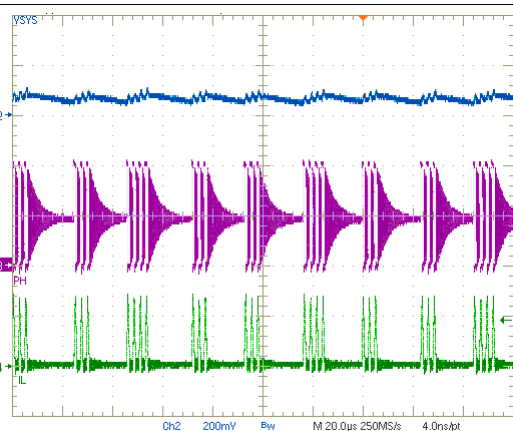
Figure 26. Charge Enable From 0x14()
