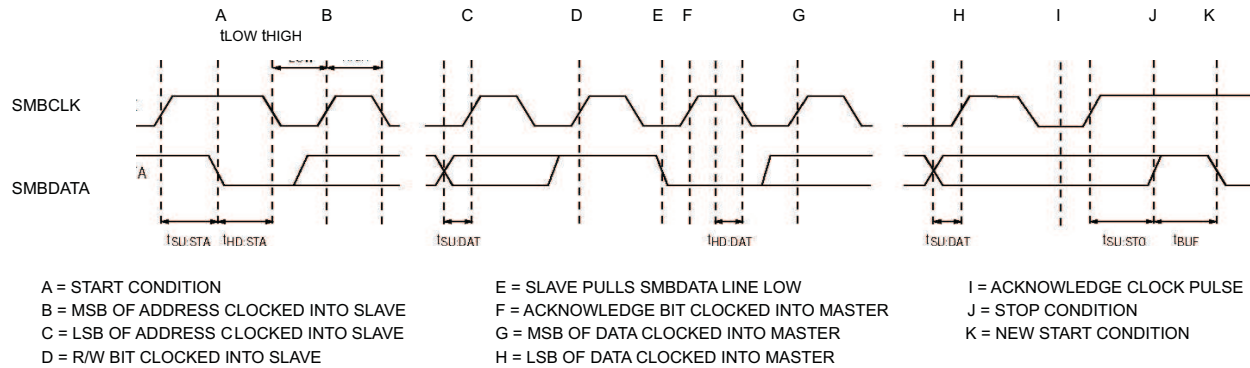
Figure 35. SMBus Read Timing
