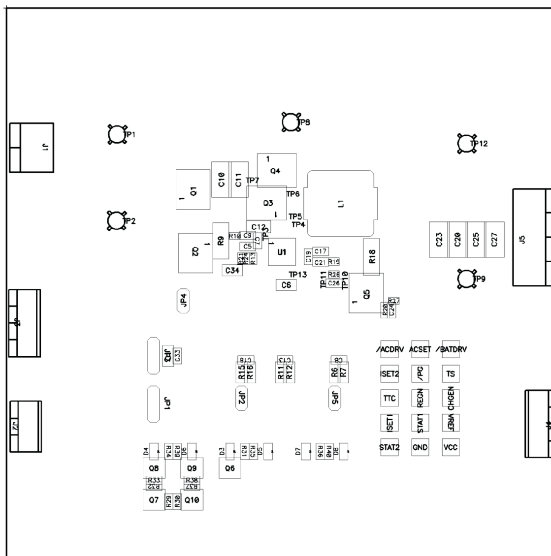
Figure 6. Top Assembly
