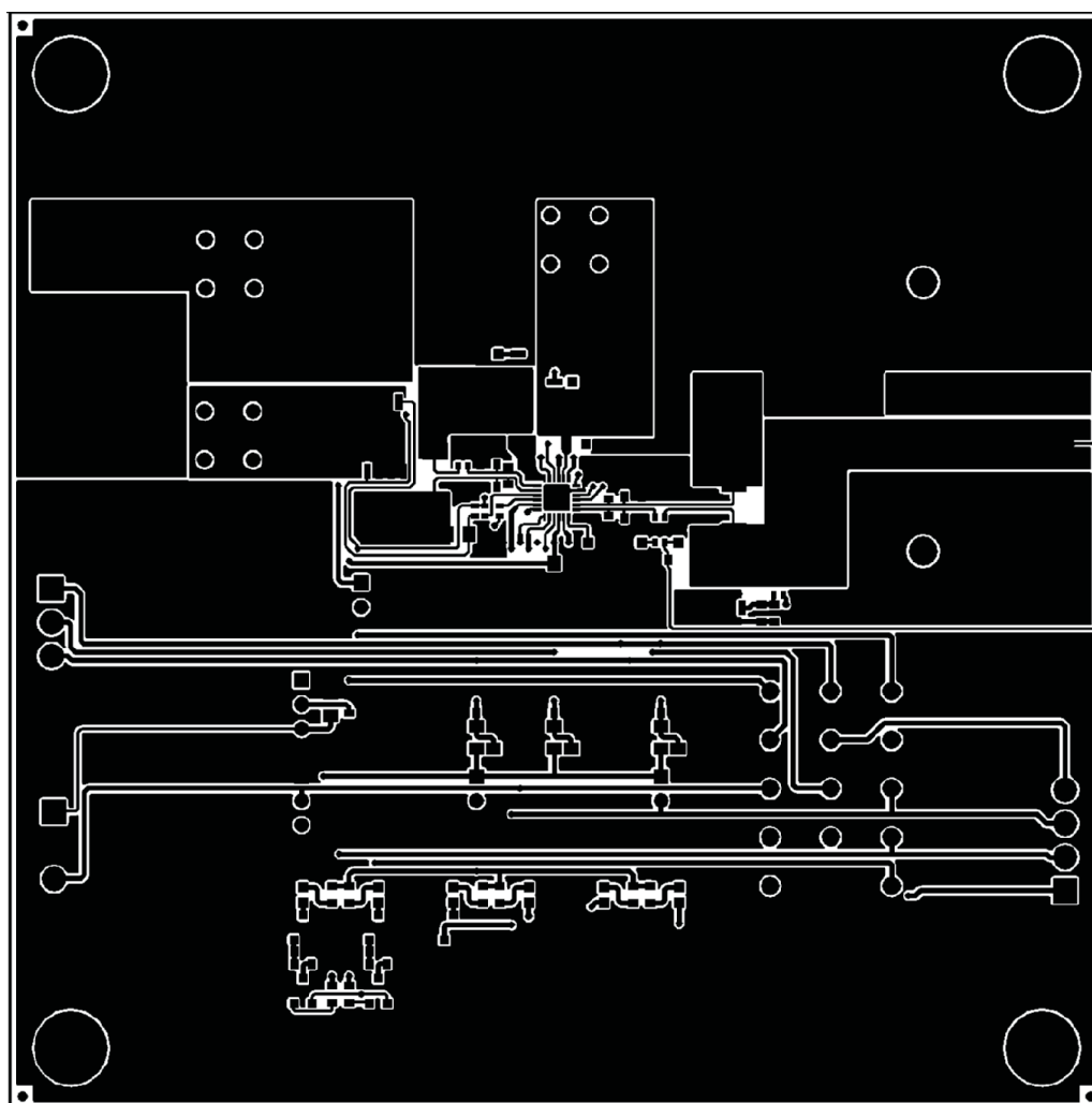
Figure 2. Top Layer
