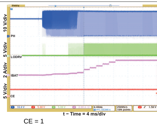
Figure 13. Current Soft-Start
