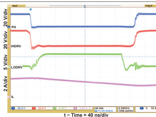
Figure 14. Continuous-Conduction-Mode Switching Waveforms
