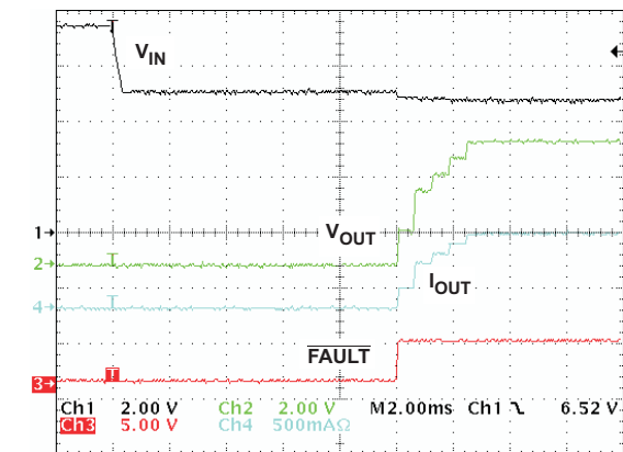
Figure 18. Recovery from OVP
