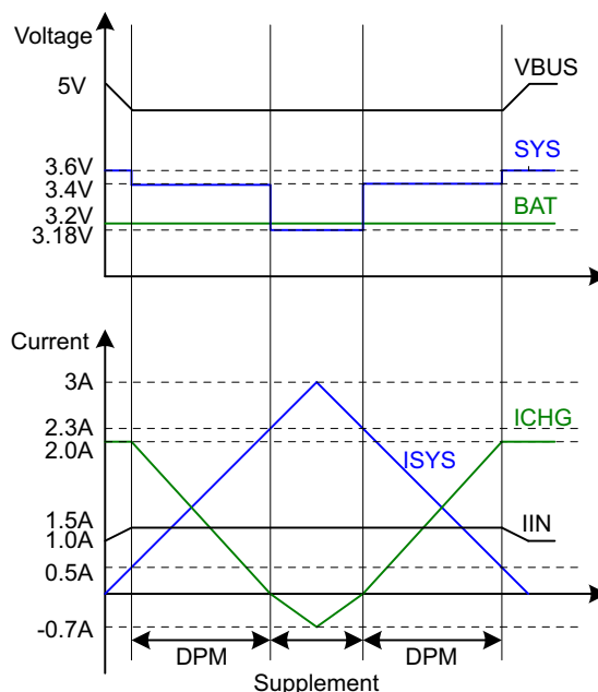
Figure 13. DPM Response
