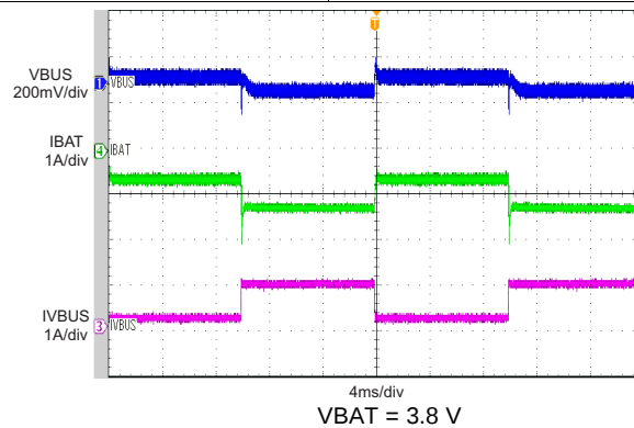
Figure 50. Load Transient During Supplement Mode
