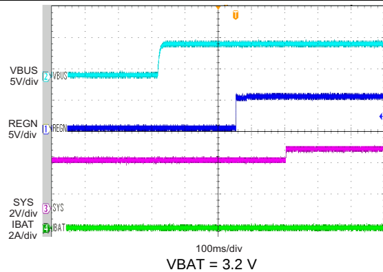
Figure 42. bq24296 Power Up with Charge Enabled
