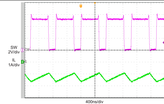
Figure 49. Input Current DPM Response without Battery
