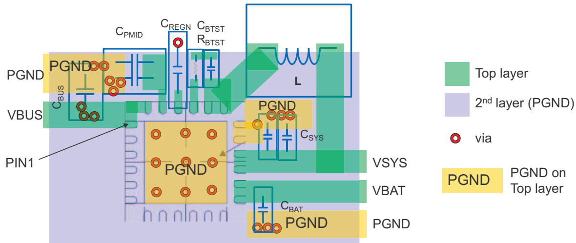
Figure 54. Layout Example
