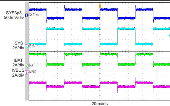
Figure 48. PFM Switching in Buck Mode
