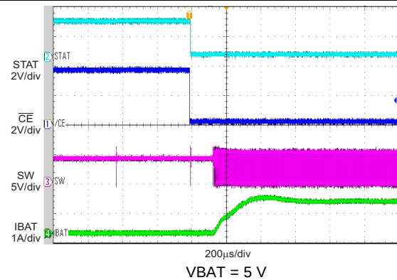
Figure 43. bq24297 Power Up with Charge Enabled
