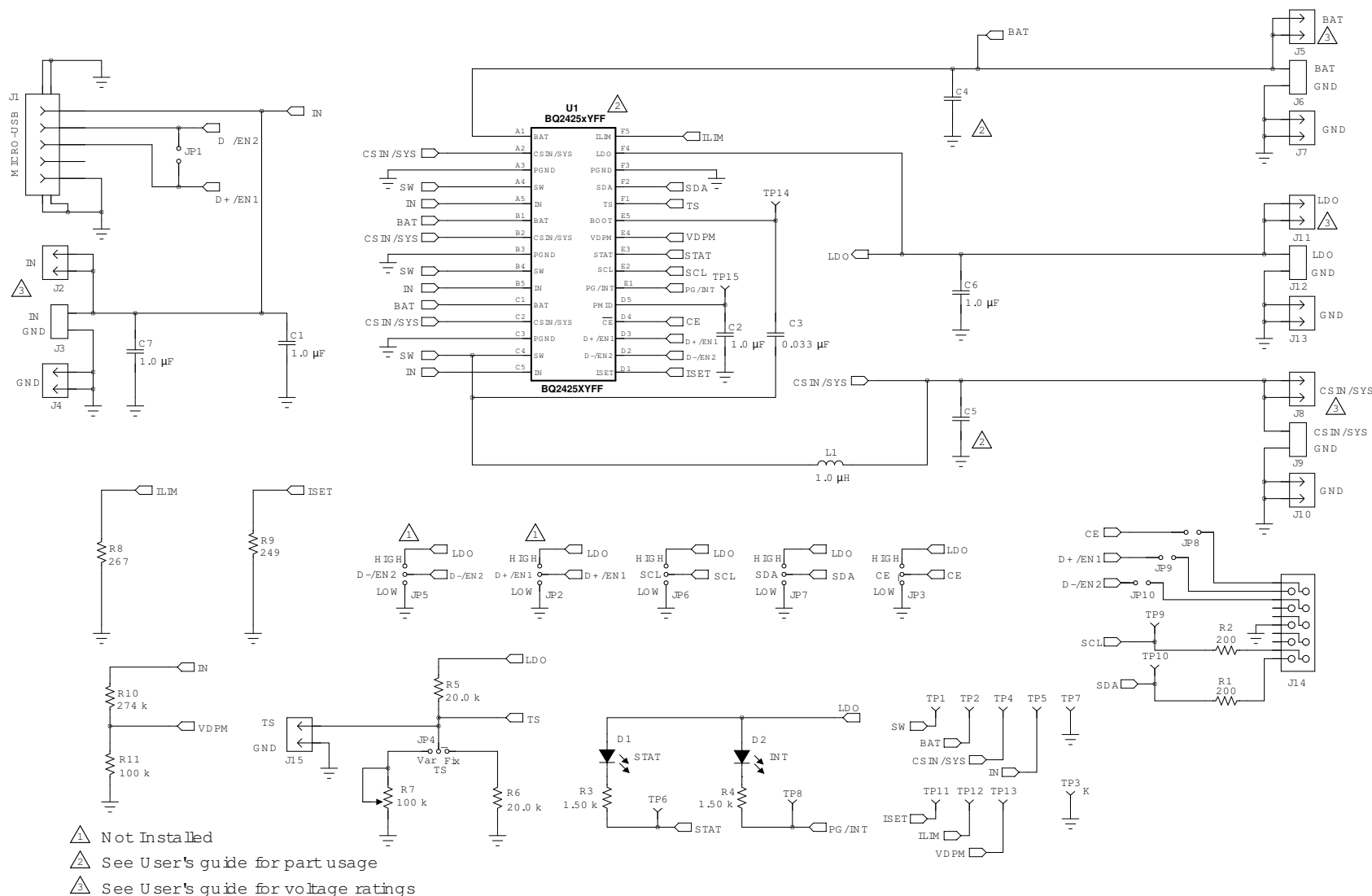
Figure 1. bq2425xEVM-150 Schematic
