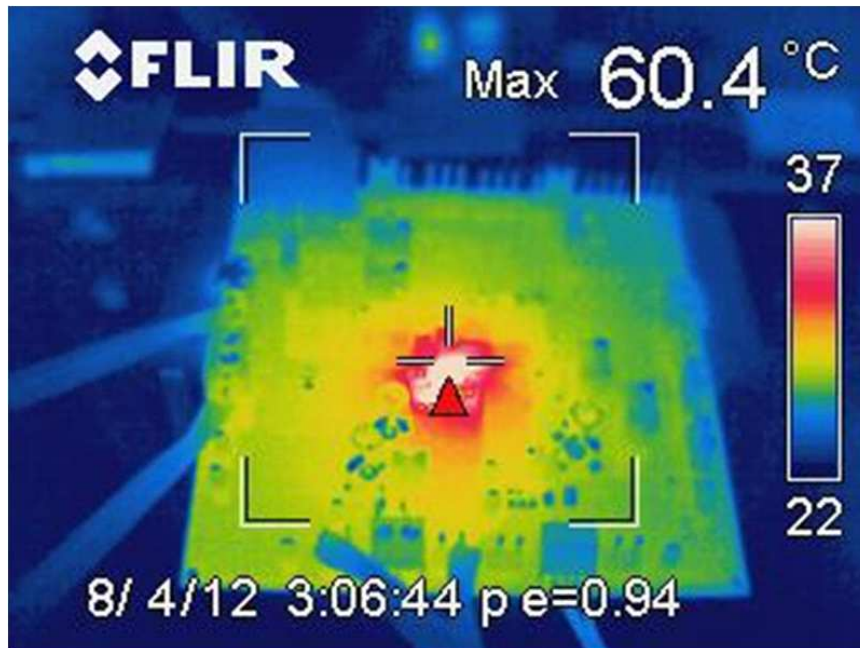
Figure 9. Thermal Image
