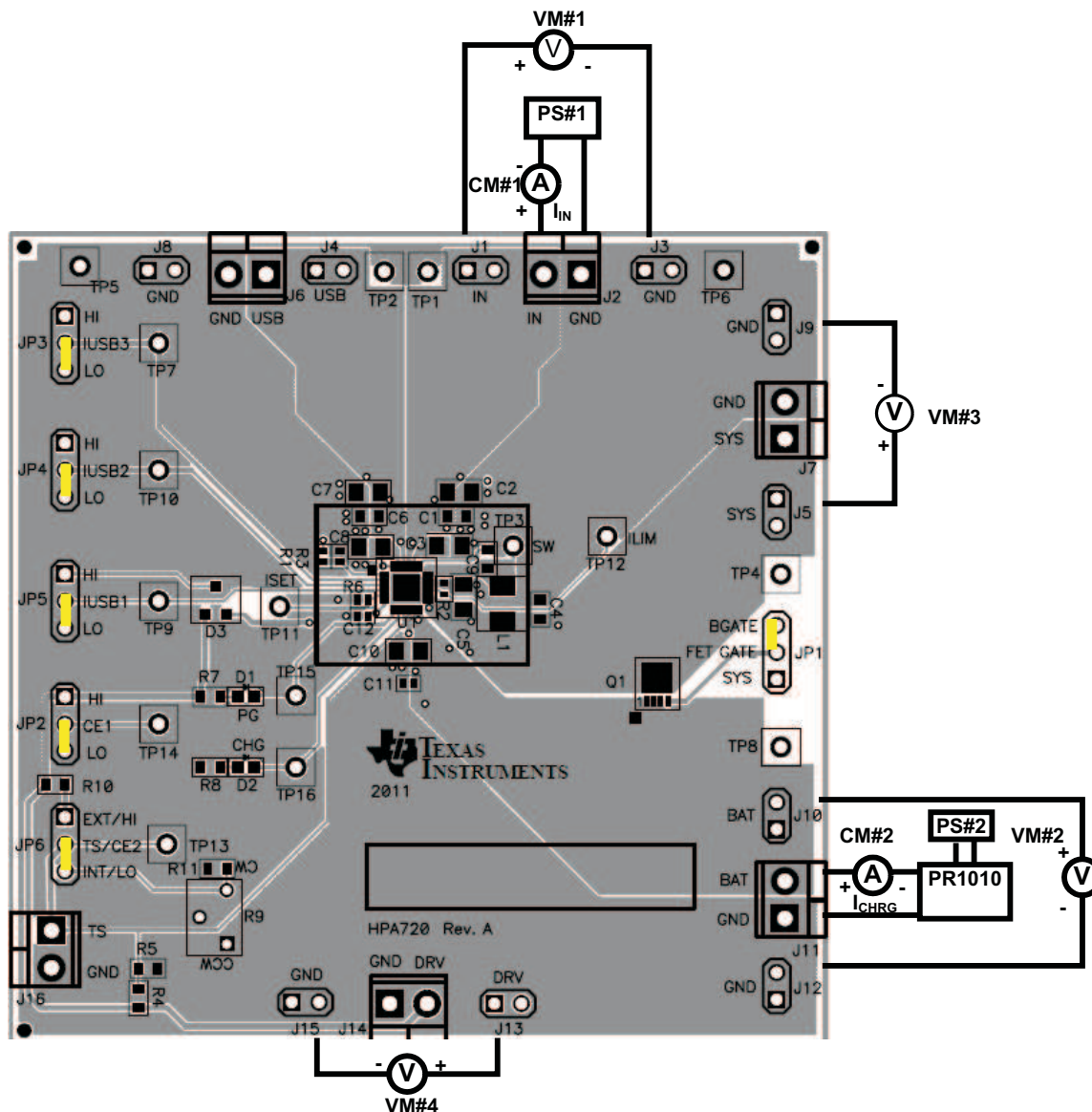
Figure 3. Original Test Setup for bq24165/166/167EVM (HPA720)
