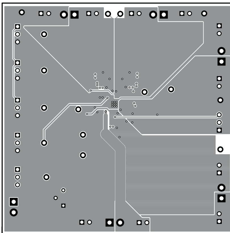
Figure 7. First Internal Layer
