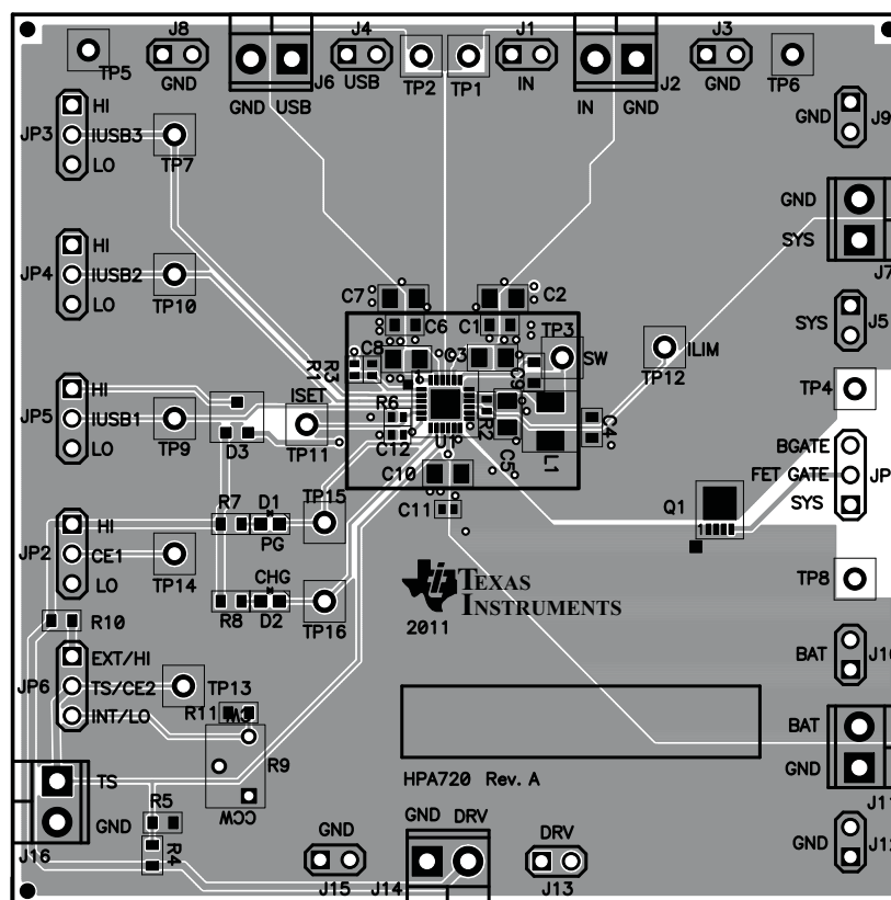
Figure 4. Top Assembly Layer
