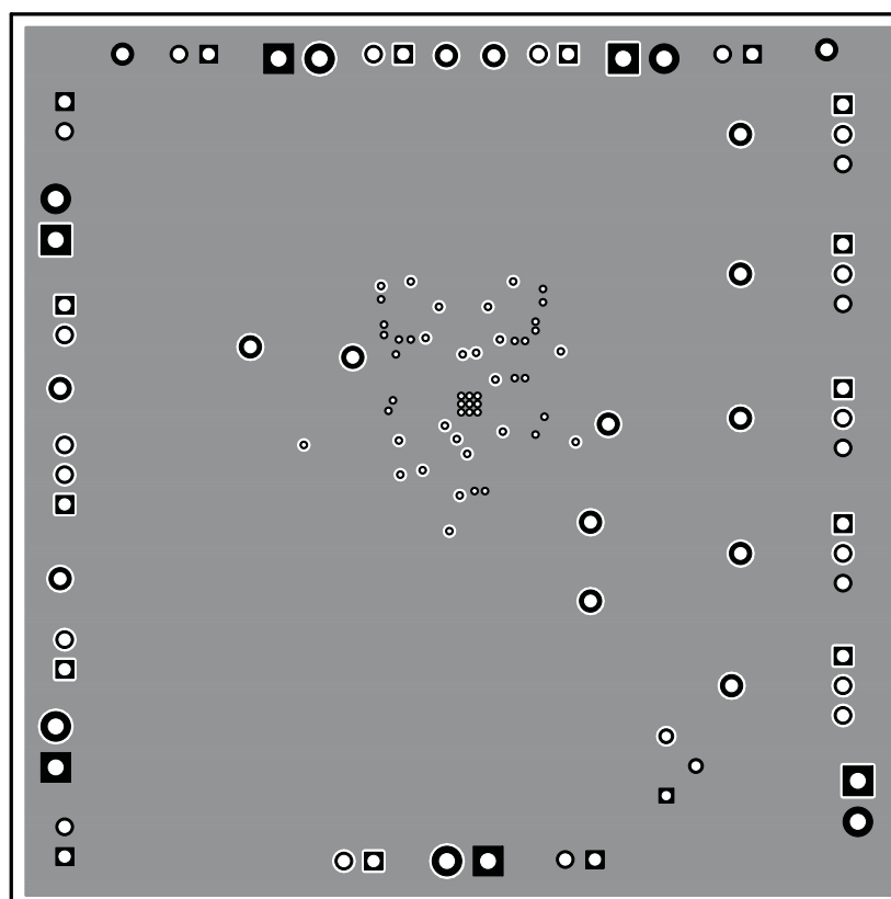
Figure 6. Bottom Layer
