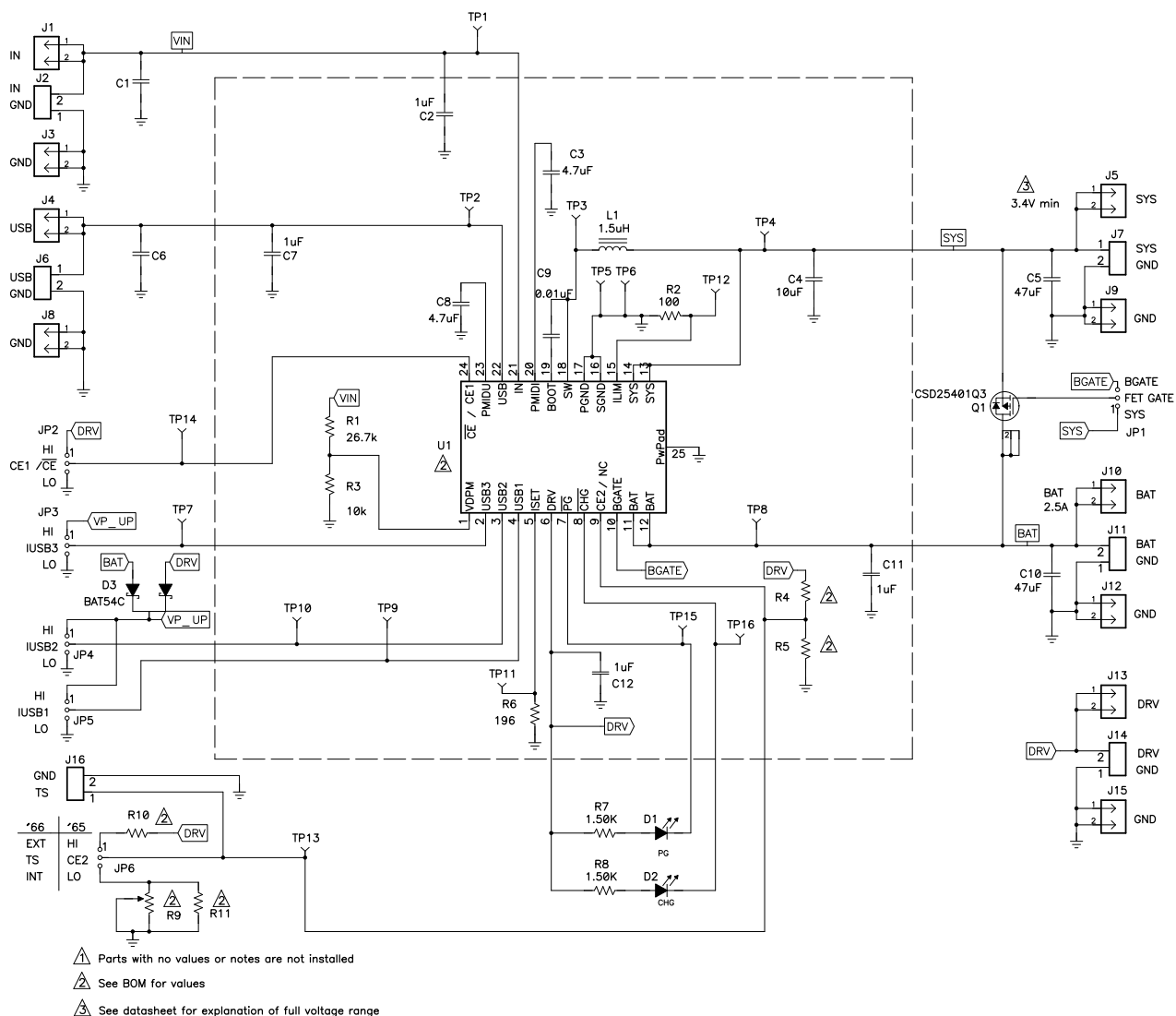
Figure 1. bq24165/166/167EVM (HPA720A) Schematic
