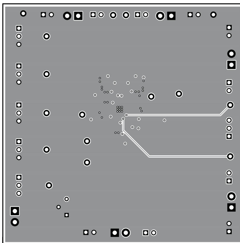
Figure 8. Second Internal Layer
