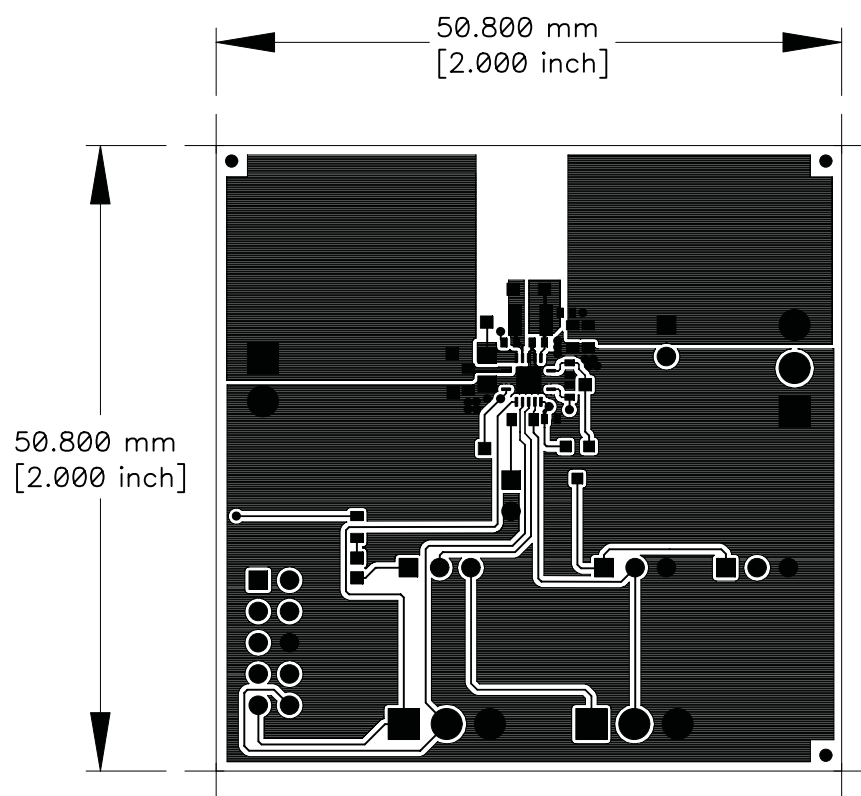
Figure 5. Top Layer
