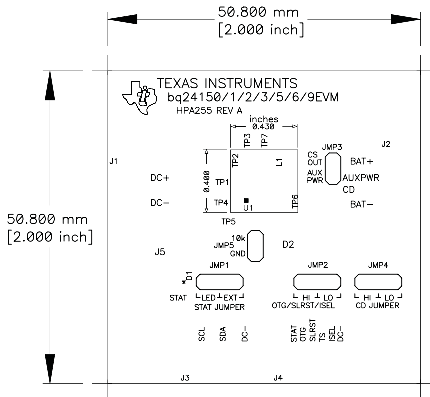
Figure 8. Top Silk
