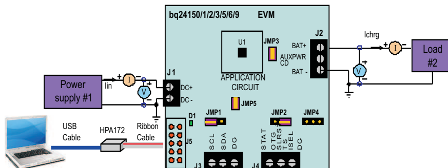
Figure 2. Original Test Setup for HPA255 (bq2415x EVM)
