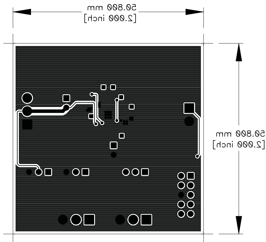
Figure 6. Bottom Layer
