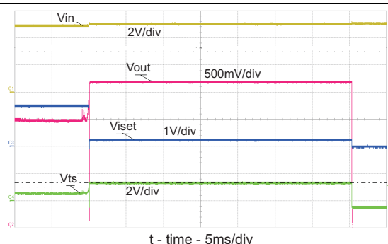
Figure 5. Battery Removal – GND Removed 1st, 42 \Omega Load
