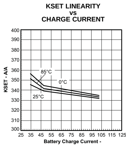
Figure 9. 2.0 < V_{(BAT)} < 3.0 V
