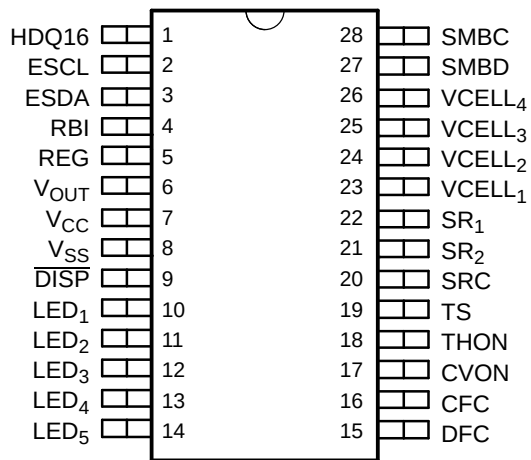
28-pin 150-mil SSOP
