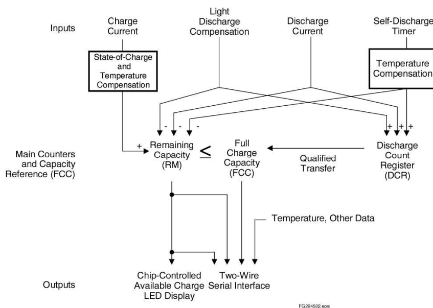
Figure 6. bq2060 Operational Overview
