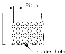
PCB Hole Layout
