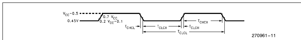
Figure 10. Clock Signal Waveform for I_{CC} Tests in Active and Idle Modes. T_{CHLH} = T_{CHCL} = 5 \text{ ns}.
