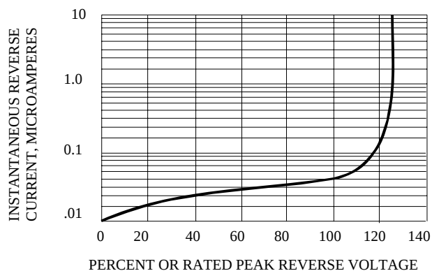
FIG. 2 - TYPICAL REVERSE CHARACTERISTICS AT T_J=25^\circ\text{C}
