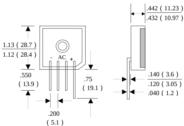
BP35-L IN LINE PIN CONFIGURATION (PLASTIC CASE)
